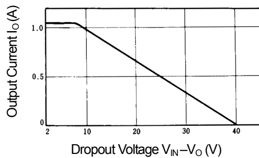
NJM78M00 Series Short Circuit Output Current
