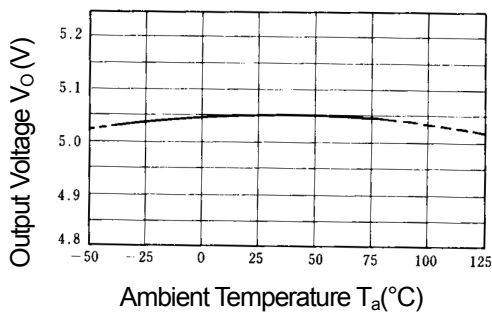
NJM78M05 Output Voltage vs. Temperature
