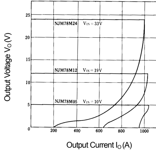
NJM78M05/M15/M24 Output Characteristics ( I_o=0.35A , T_j=25^\circ C )
