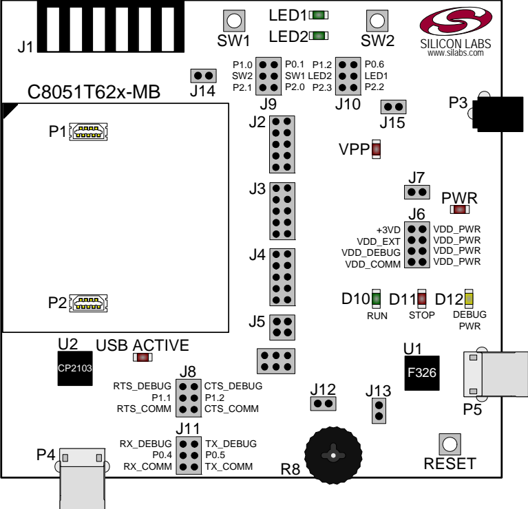
Figure 3. C8051T62x Motherboard
