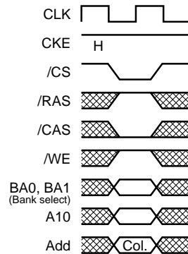
Column Address and Read Command
