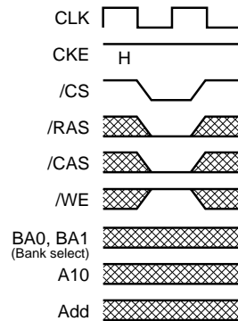
CBR (auto) Refresh Command
