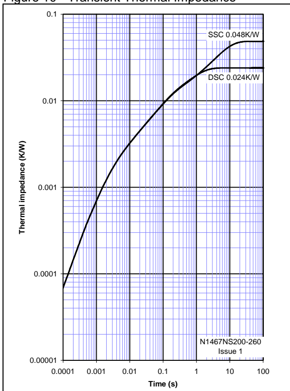
Figure 10 - Transient Thermal Impedance
