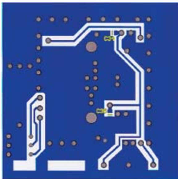
Figure 25: PC Board Layout Bottom View
