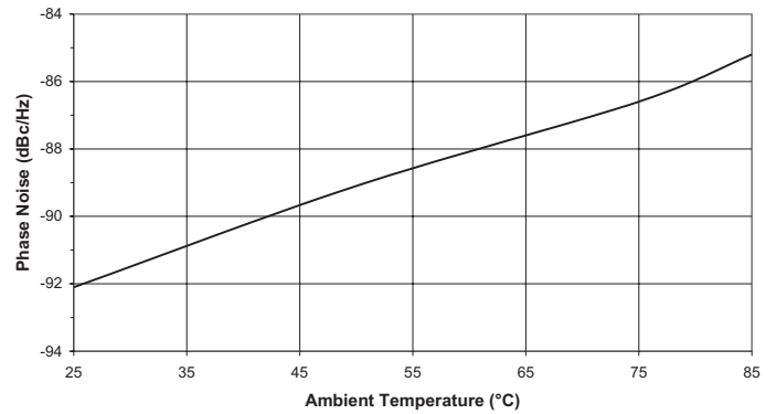
Figure 8: Typical Phase Noise at 10 kHz Offset vs. Ambient Temperature ( V_{DD} = +5\text{ V} , f_{LO2} = 1042\text{ MHz} )
