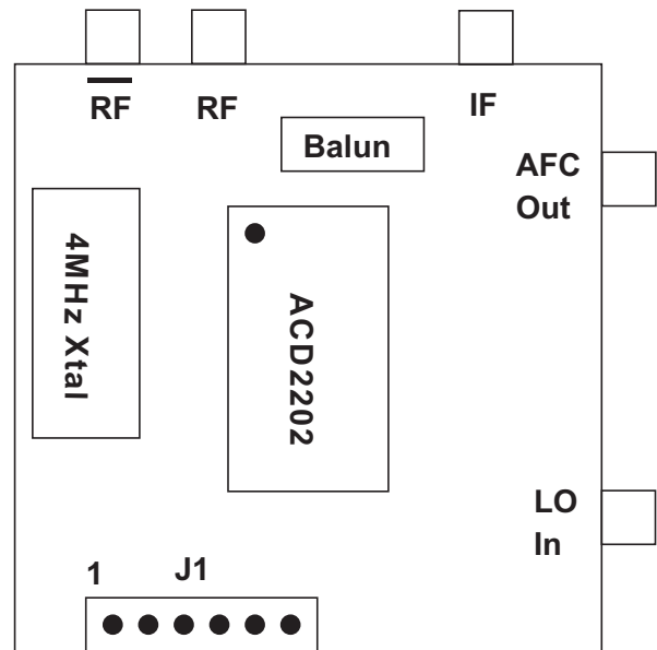
Figure 26 Evaluation Fixture
