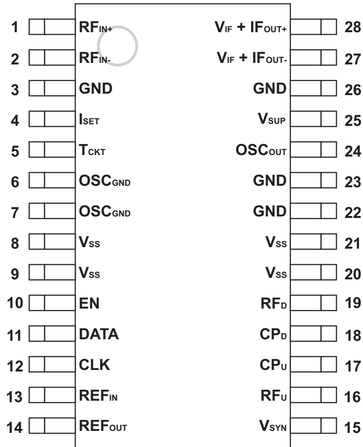
Figure 3: Pinout
