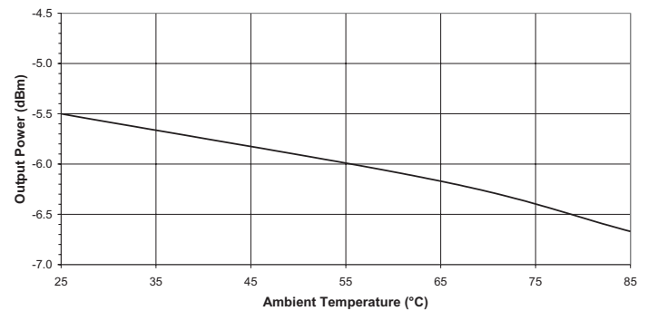
Figure 10: Typical Local Oscillator Output Power vs. Ambient Temperature ( V_{DD} = +5\text{ V} , f_{LO2} = 1042\text{ MHz} )
