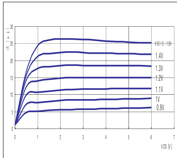
Fig.3. Output characteristics
