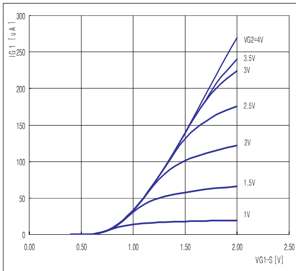
Fig.2 Transfer characteristics
