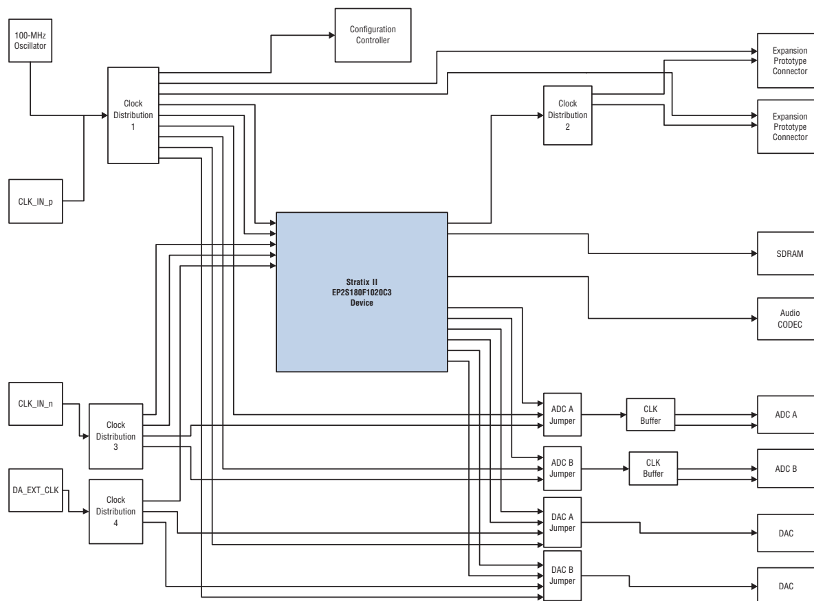
Figure 2–3. Clock Distribution
