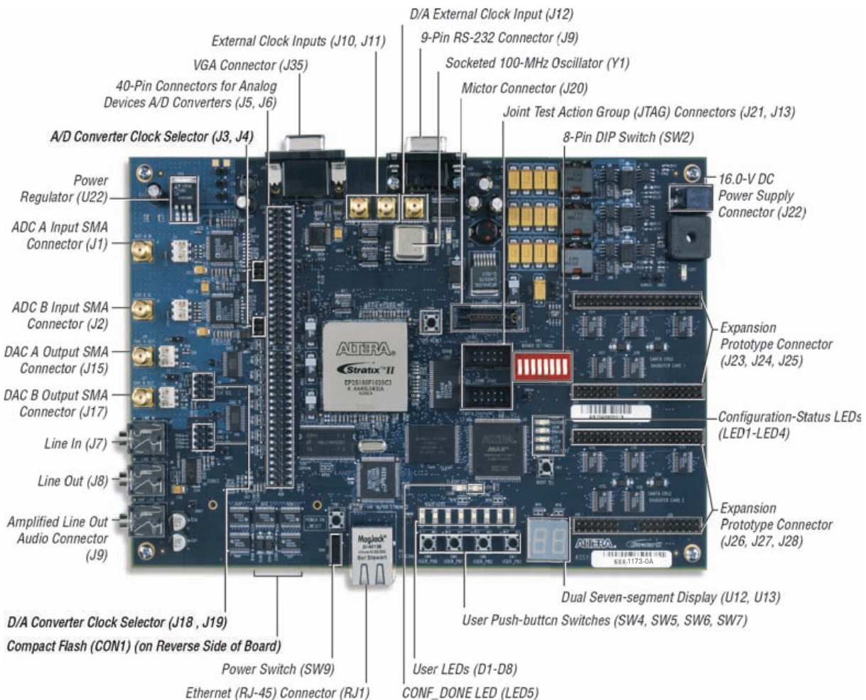
Figure 2–1. Stratix II EP2S180 DSP Development Board Components nterfaces
