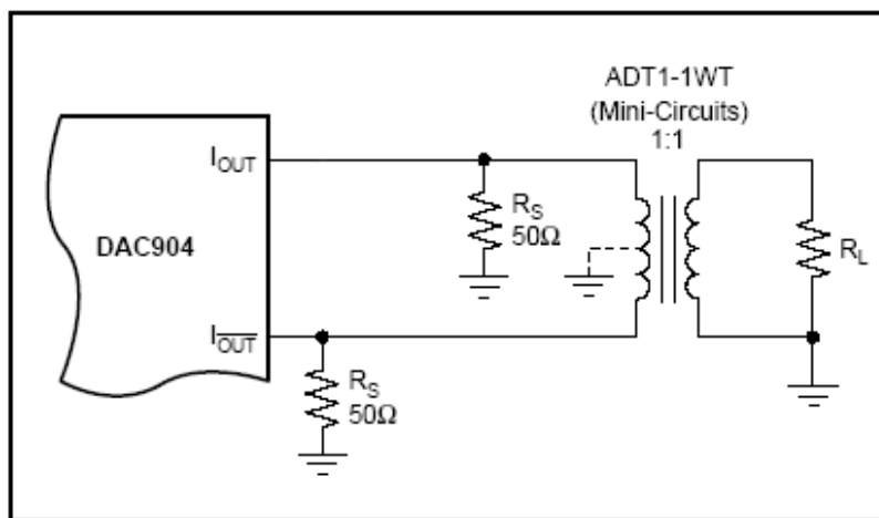
Figure 2-5. On-Board Circuitry after D/A Converter
