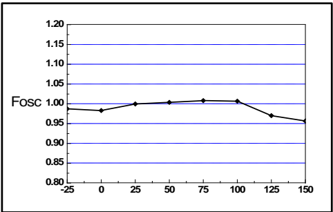
Figure 1. Operating Frequency
