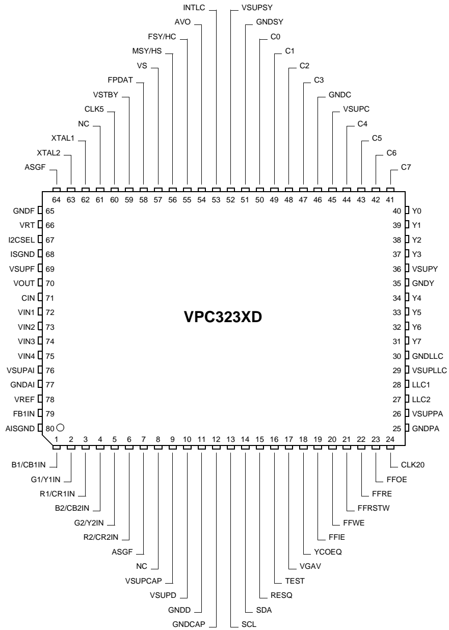
Fig. 4-2: 80-pin PQFP package
