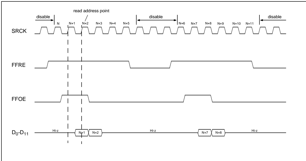
Fig. 4-16: Field memory read cycle timing
