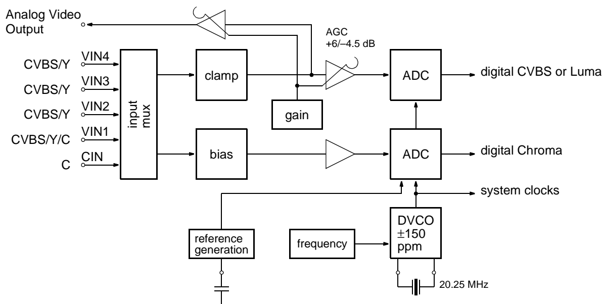
Fig. 2–1: Analog front-end
