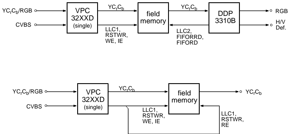
Fig. 2–21: Typical configurations with single VPC 32xxD
