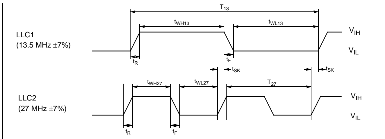
Fig. 4–18: Line-locked clock output pins
