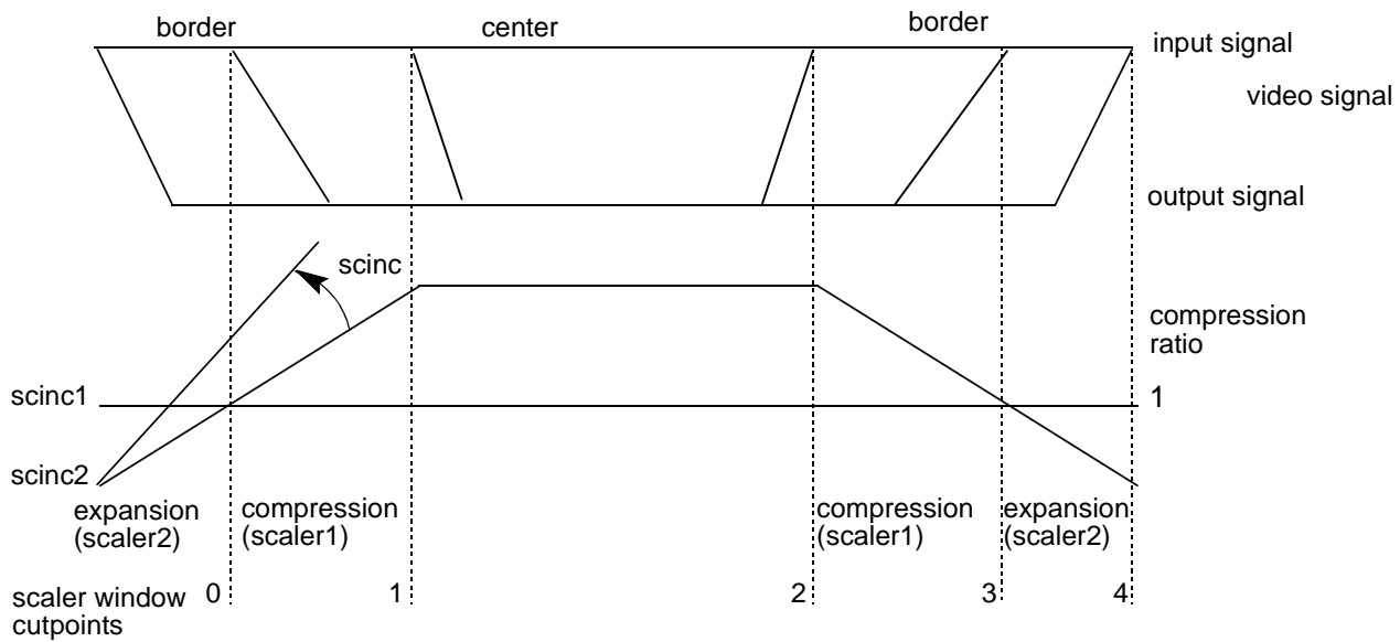
Fig. 3–2: Scaler operation for ‘panorama’ mode at 13.5 MHz
