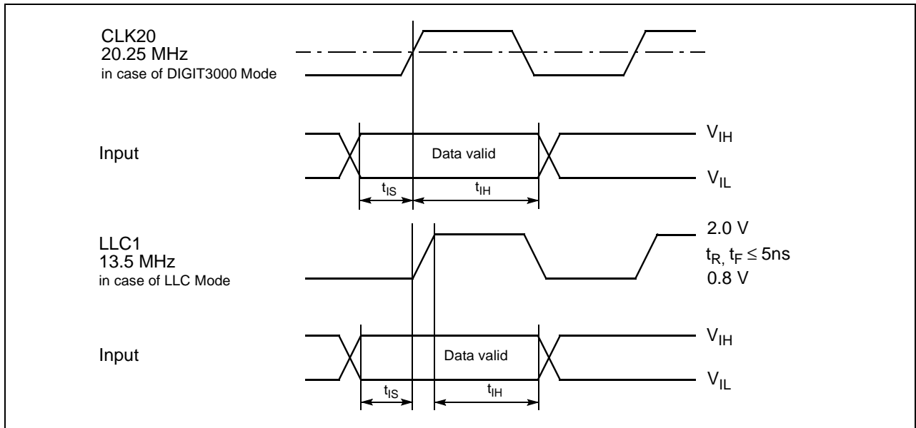
Fig. 4–17: Sync, control, and data inputs
