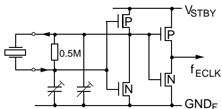
Fig. 4-7: Input/Output Pins XTAL1, XTAL2
