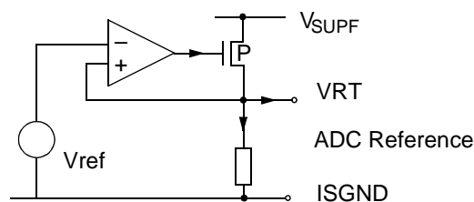
Fig. 4-8: Pins VRT, ISGND and VREF, AISGND
