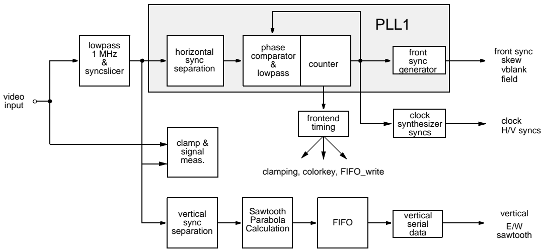
Fig. 2–18: Sync separation block diagram
