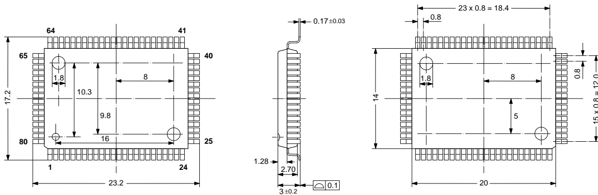
Fig. 4–1: 80-Pin Plastic Quad Flat Package (PQFP80)
