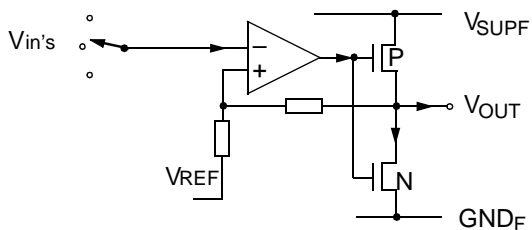
Fig. 4-6: Output pin VOUT
