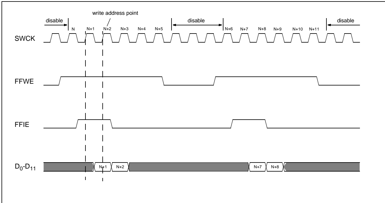
Fig. 4-15: Field memory write cycle timing
