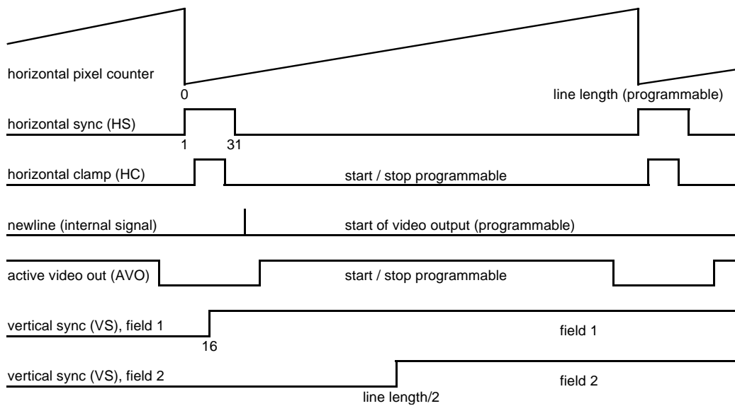
Fig. 2–16: Horizontal timing for line-locked mode
