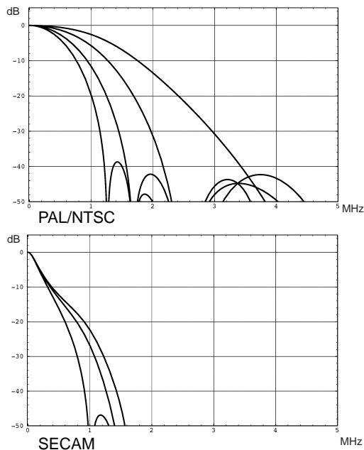
Fig. 2-5: Frequency response of chroma filters
