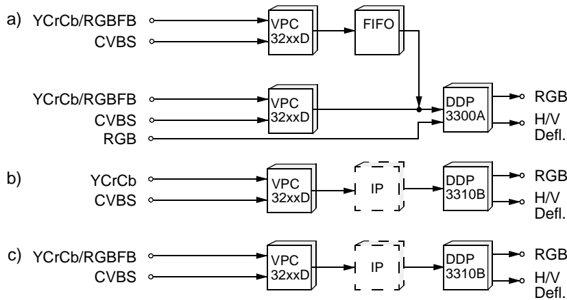
Fig. 1–2: VPC 32xxD applications
