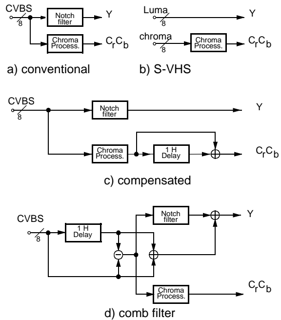
Fig. 2-6: NTSC color decoding options
