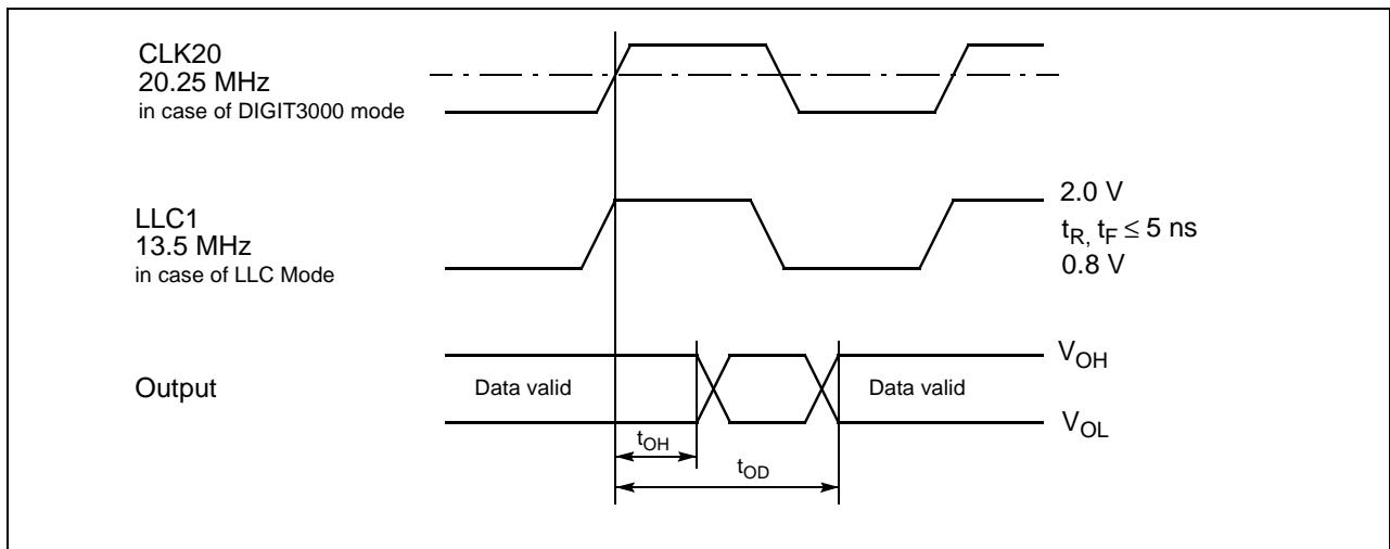
Fig. 4–14: Sync, control, and data outputs
