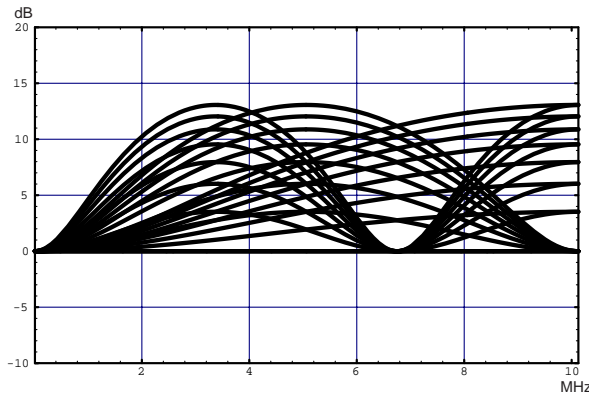
Fig. 2-13: Peaking characteristics
