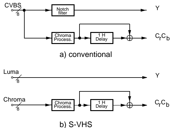
Fig. 2-7: PAL color decoding options
