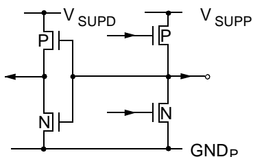
Fig. 4-4: Output pins C0-C7, Y0-Y7, FSY, MSY, HC, AVO, VS, INTLC, HS, LLC1, LLC2, CLK20, FFWE, FFIE, FFRD, RSTWR
