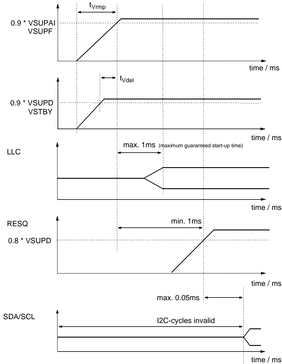
Fig. 4-13: Power-Up sequence
