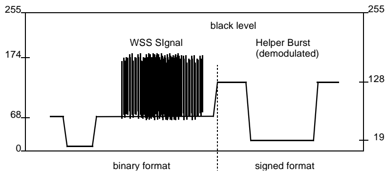
Fig. 2–17: PAL+ helper reference line output signal
