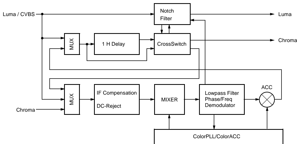
Fig. 2-4: Color decoder
