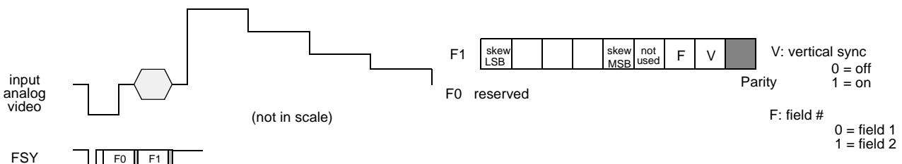
Fig. 2–19: Front sync format
