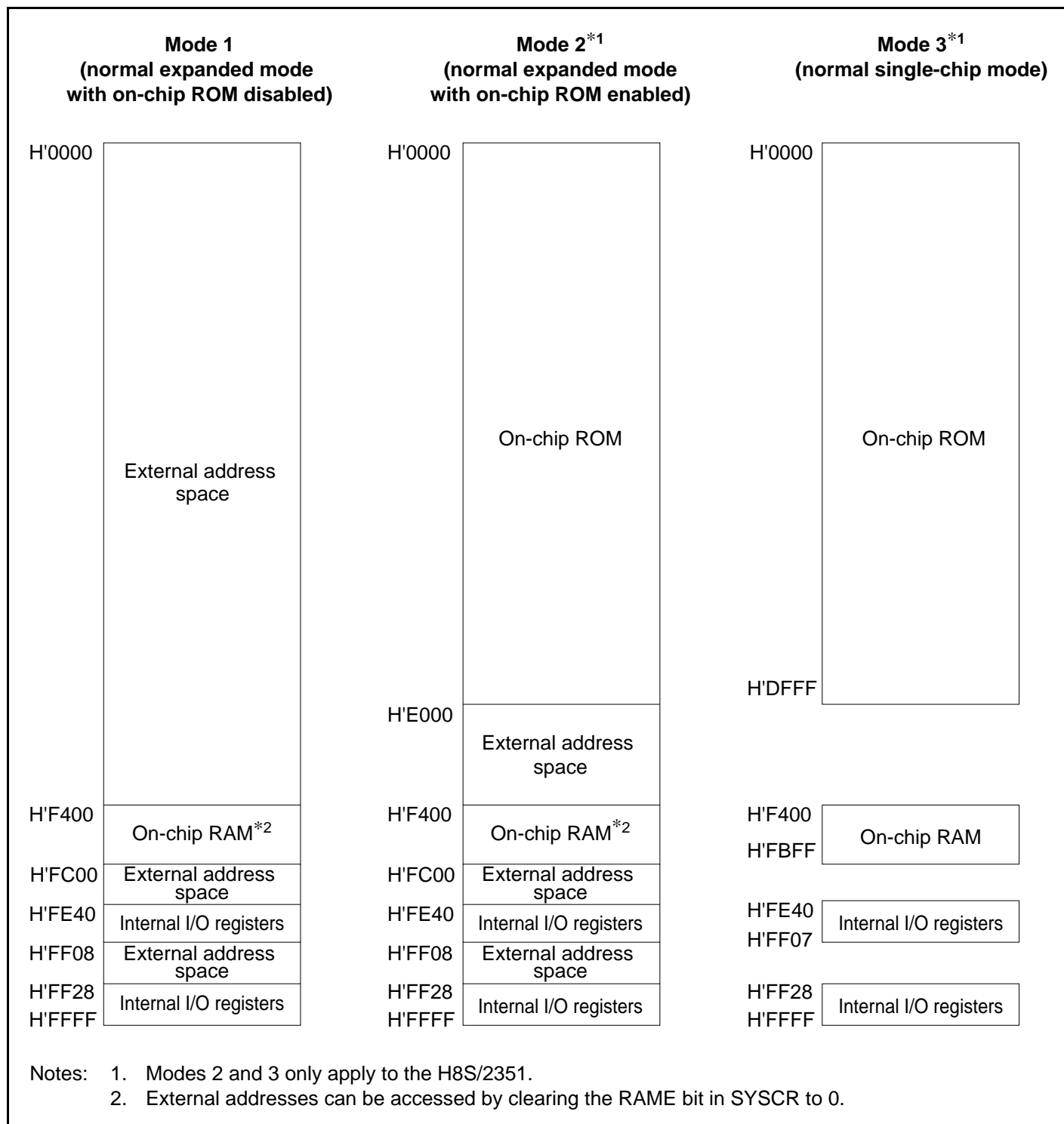
Figure 3.1 Memory Map in Each Operating Mode
