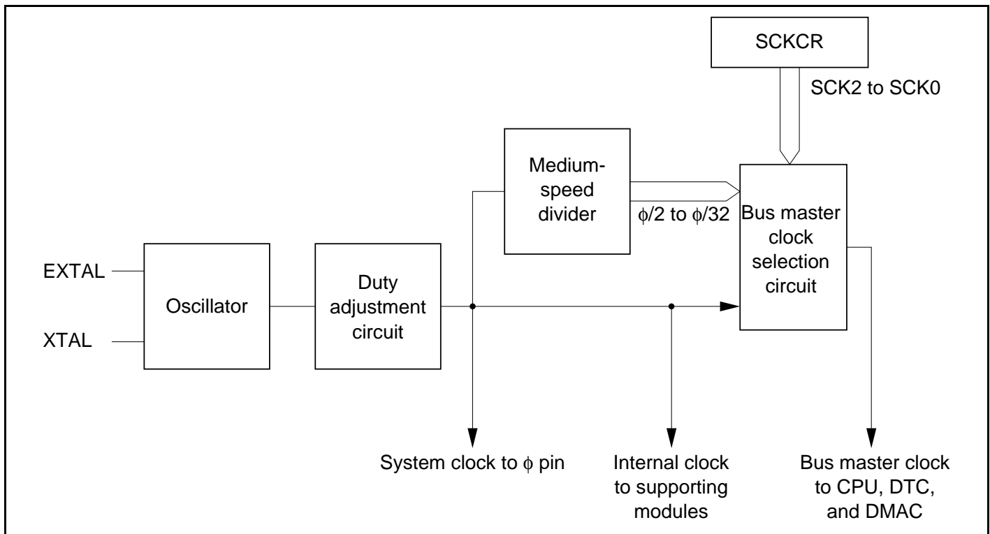
Figure 19.1 Block Diagram of Clock Pulse Generator
