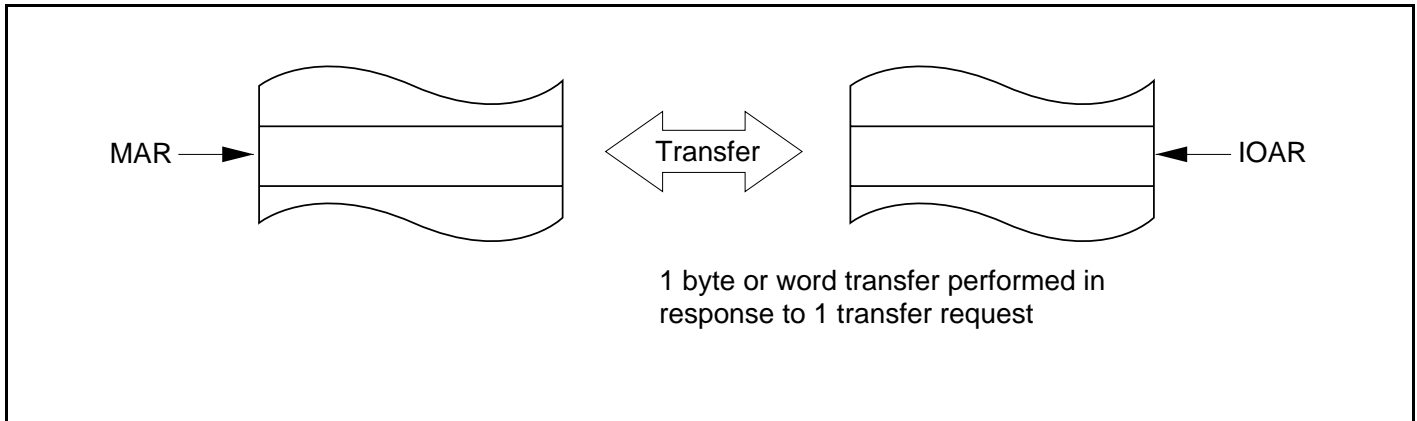
Figure 7.5 Operation in Idle Mode
