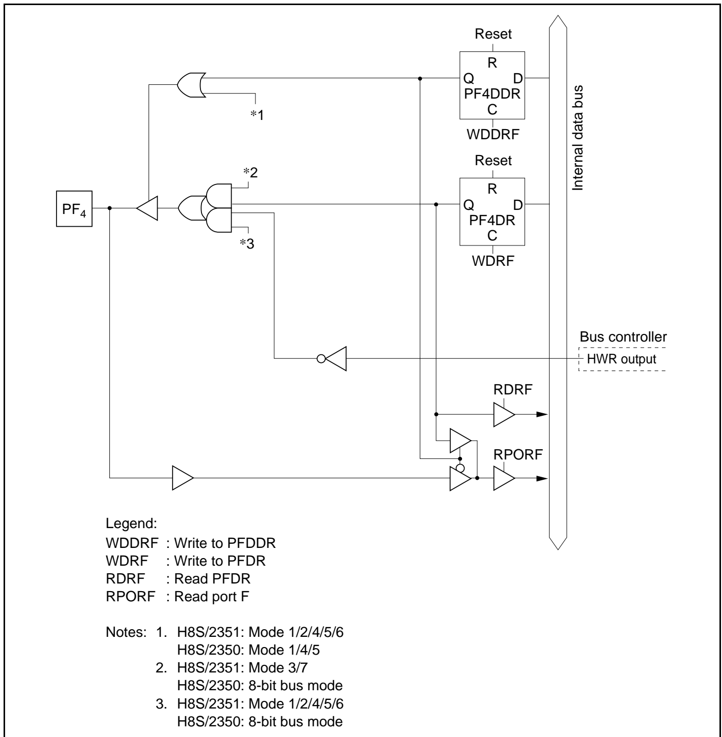
Figure C.12 (e) Port F Block Diagram (Pin PF 4 )
