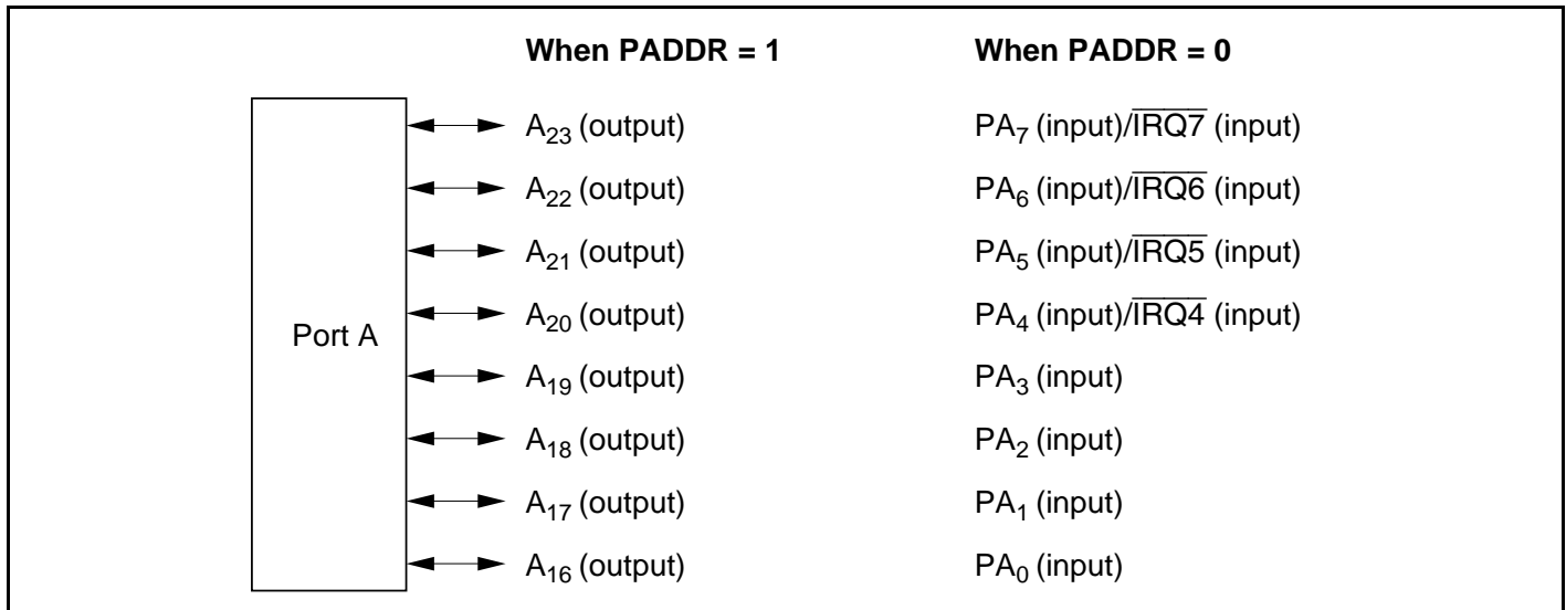
Figure 9.10 Port A Pin Functions (Mode 6)
