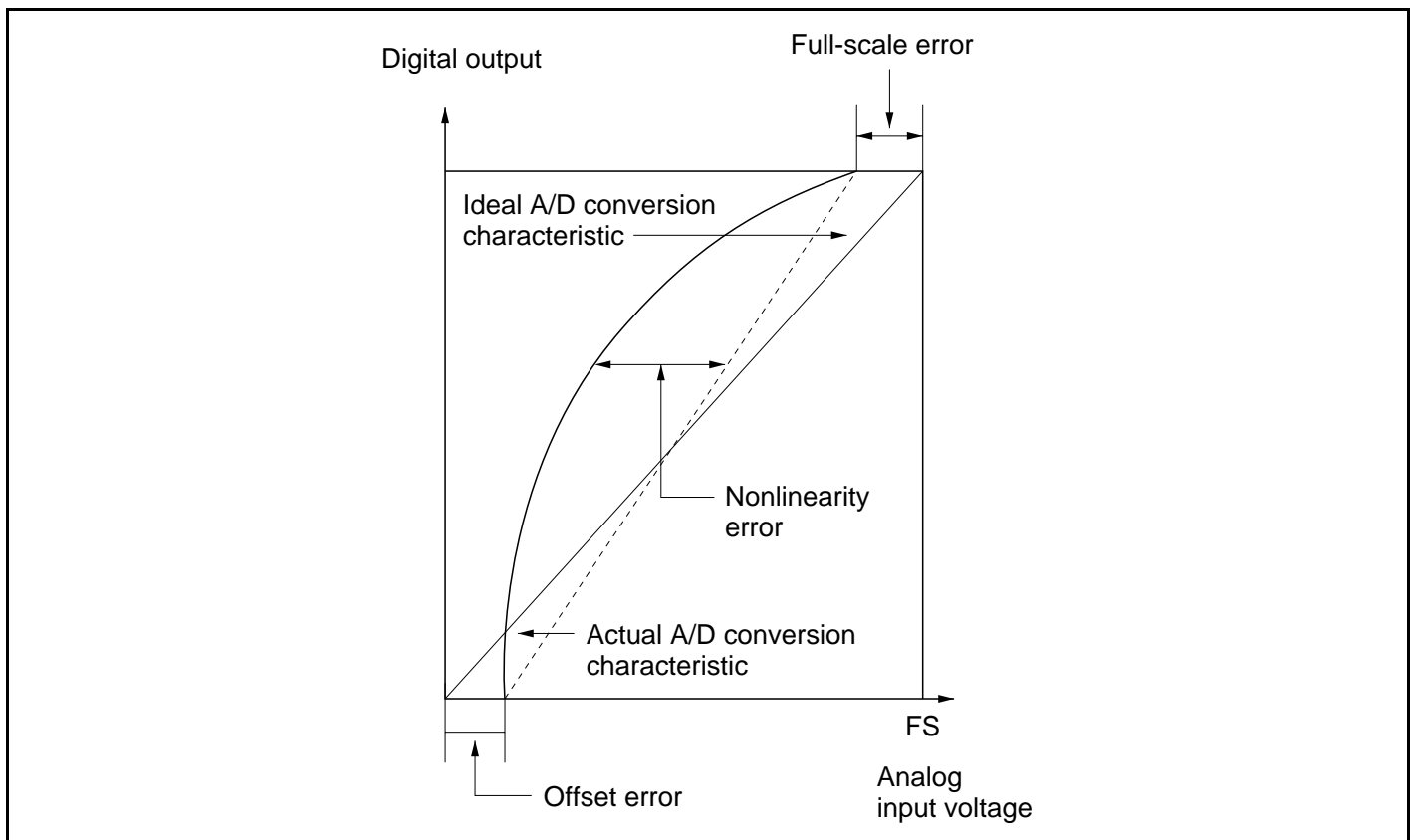
Figure 15.10 A/D Conversion Precision Definitions (2)
