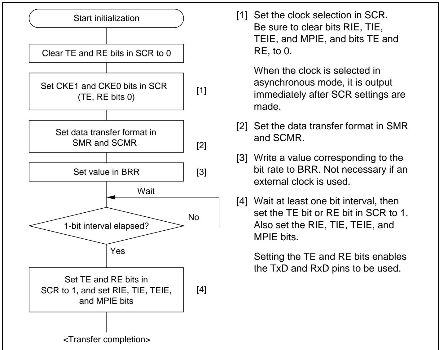
Figure 13.4 Sample SCI Initialization Flowchart
