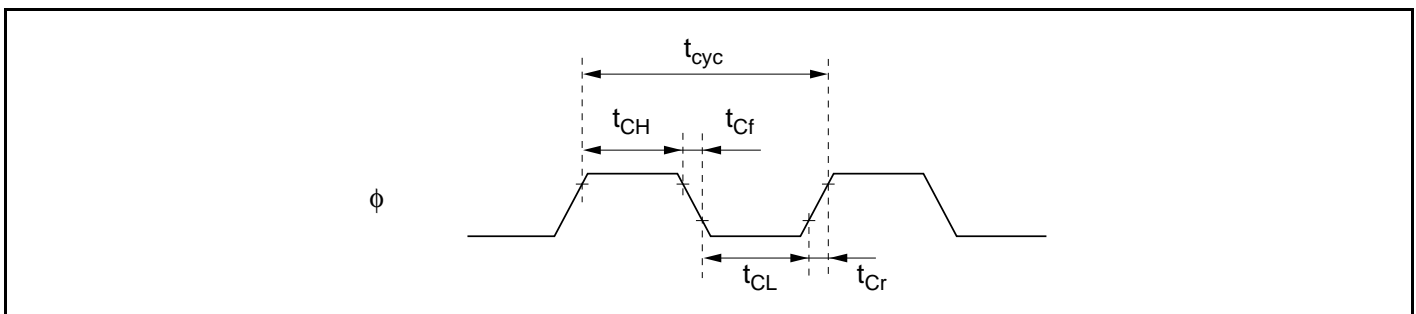
Figure 21.4 System Clock Timing
