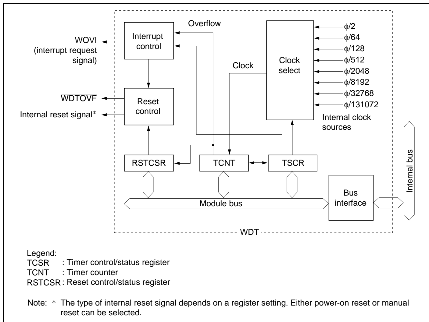
Figure 12.1 Block Diagram of WDT
