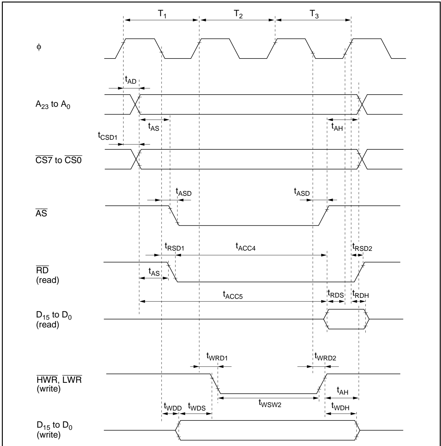
Figure 21.9 Basic Bus Timing (Three-State Access)
