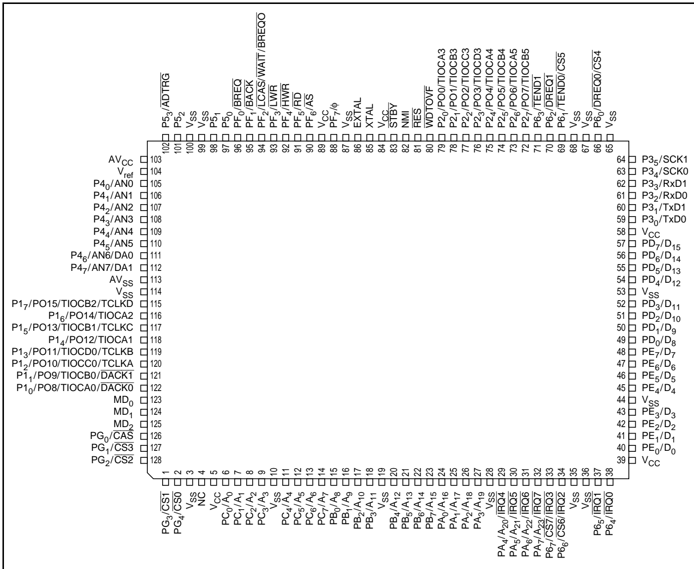
Figure 1.3 Pin Arrangement (FP-128: Top View)
