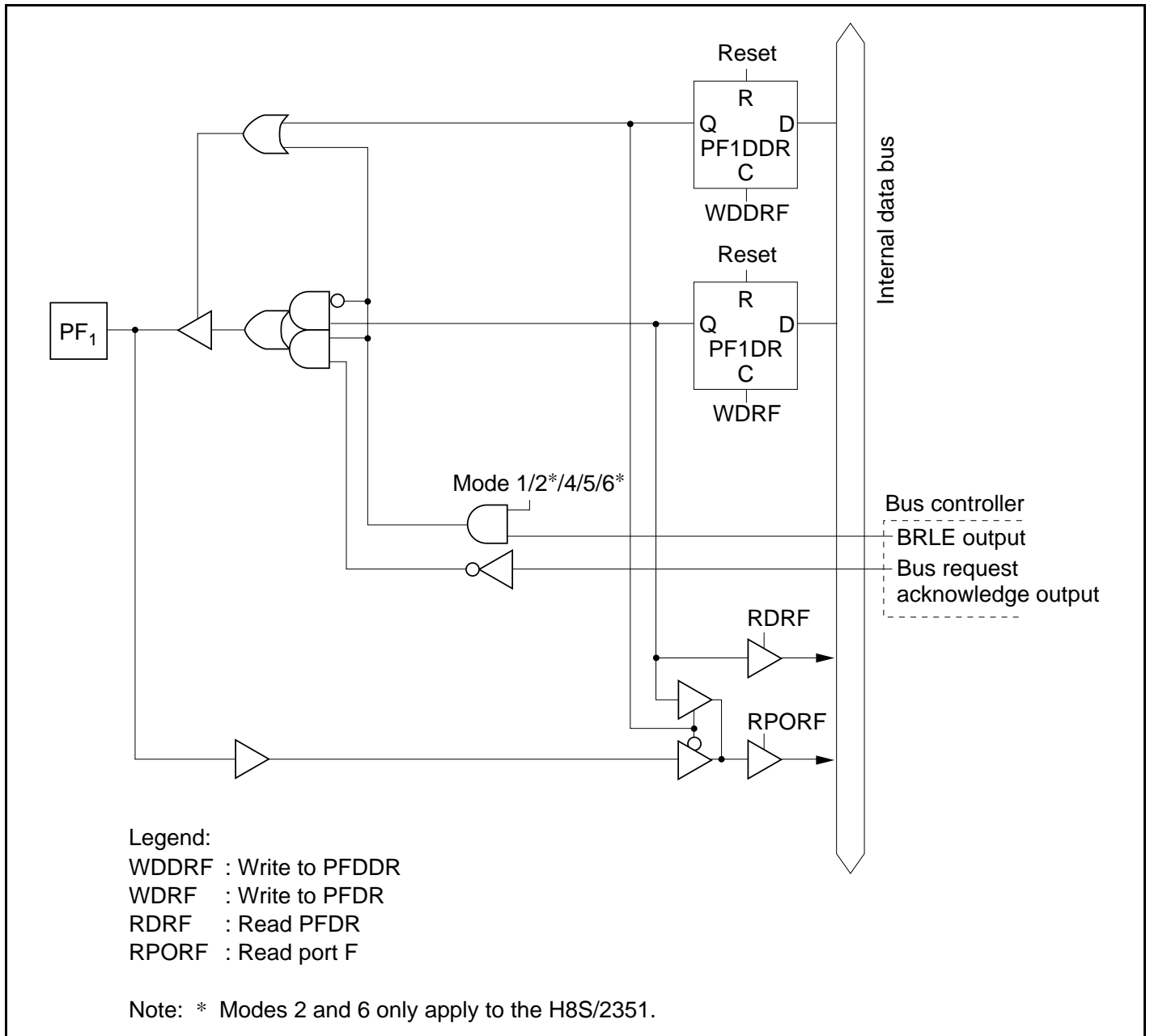
Figure C.12 (b) Port F Block Diagram (Pin PF 1 )
