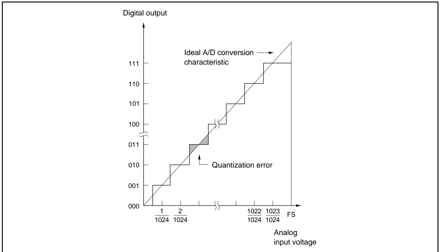
Figure 15.9 A/D Conversion Precision Definitions (1)
