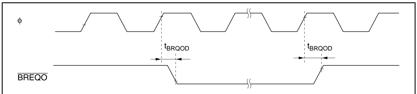
Figure 21.17 External Bus Request Output Timing
