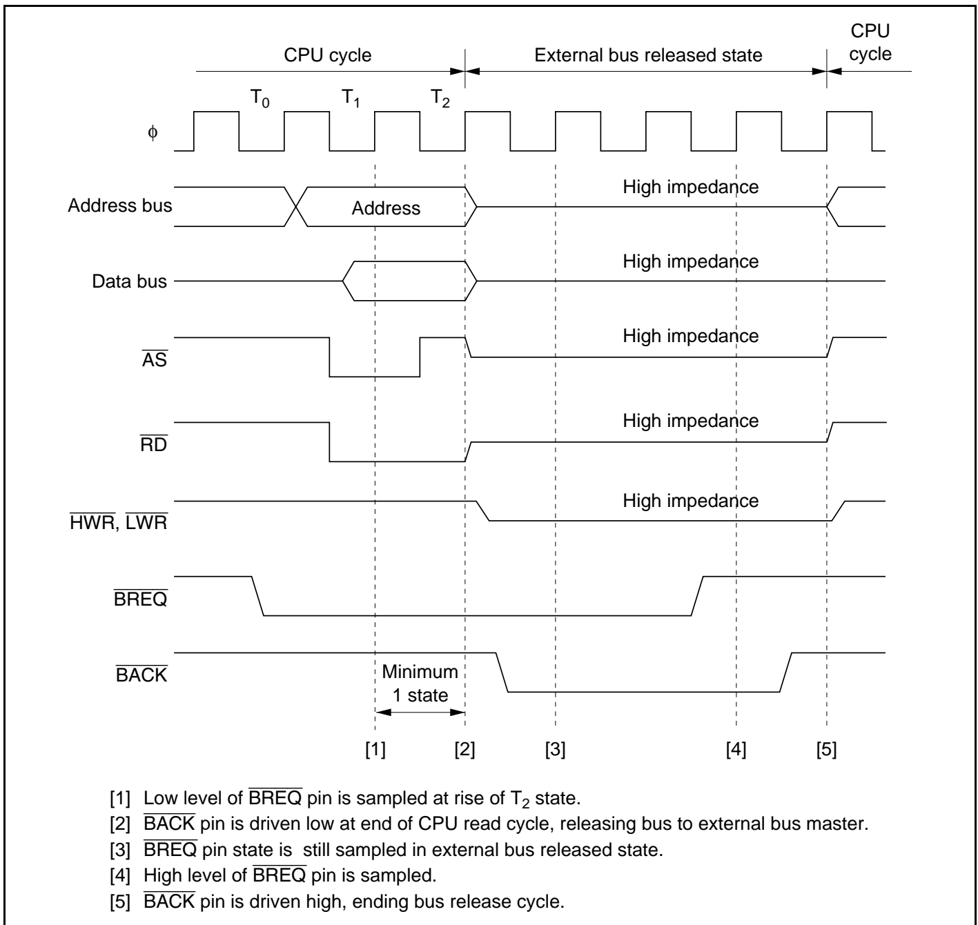
Figure 6.37 Bus-Released State Transition Timing
