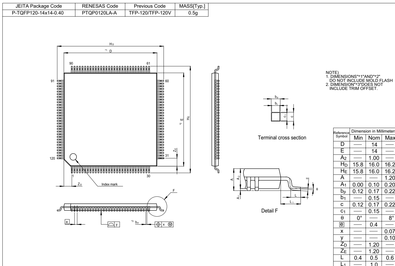
Figure H.1 TFP-120 Package Dimensions
