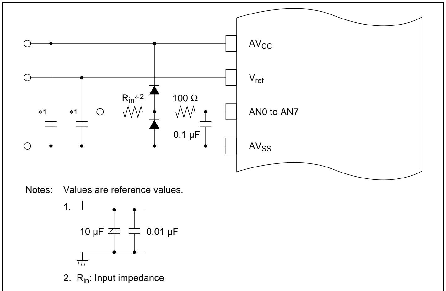
Figure 15.7 Example of Analog Input Protection Circuit
