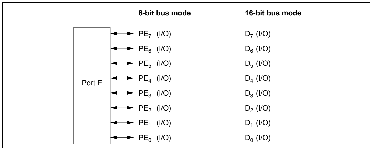
Figure 9.23 Port E Pin Functions (Modes 1, 2, and 4 to 6)
