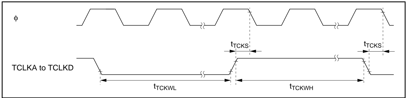
Figure 21.25 TPU Clock Input Timing
