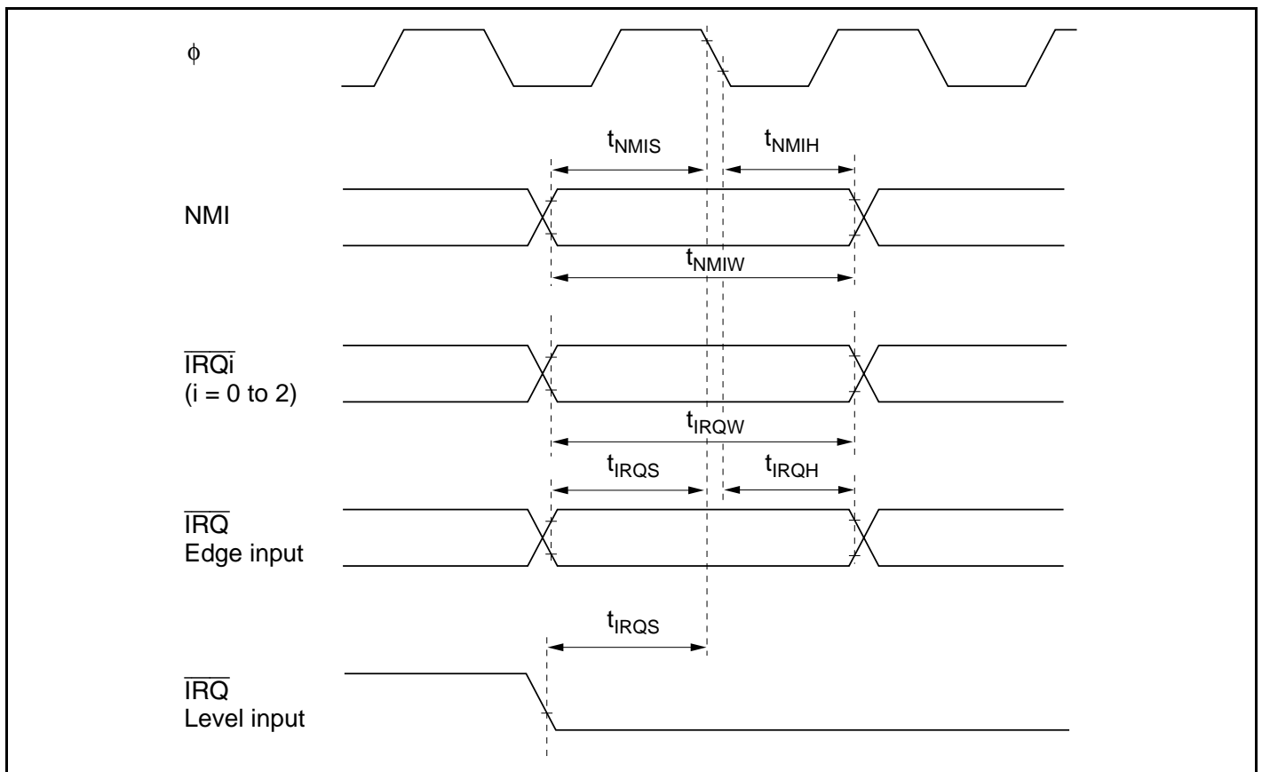
Figure 21.7 Interrupt Input Timing
