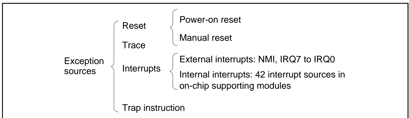
Figure 4.1 Exception Sources
