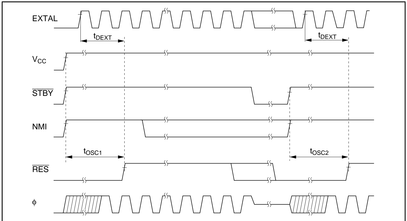
Figure 21.5 Oscillator Settling Timing
