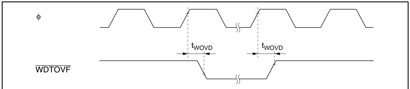
Figure 21.26 WDT Output Timing
