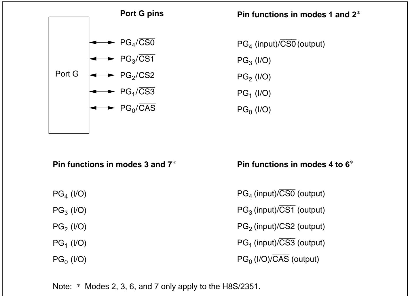
Figure 9.26 Port G Pin Functions
