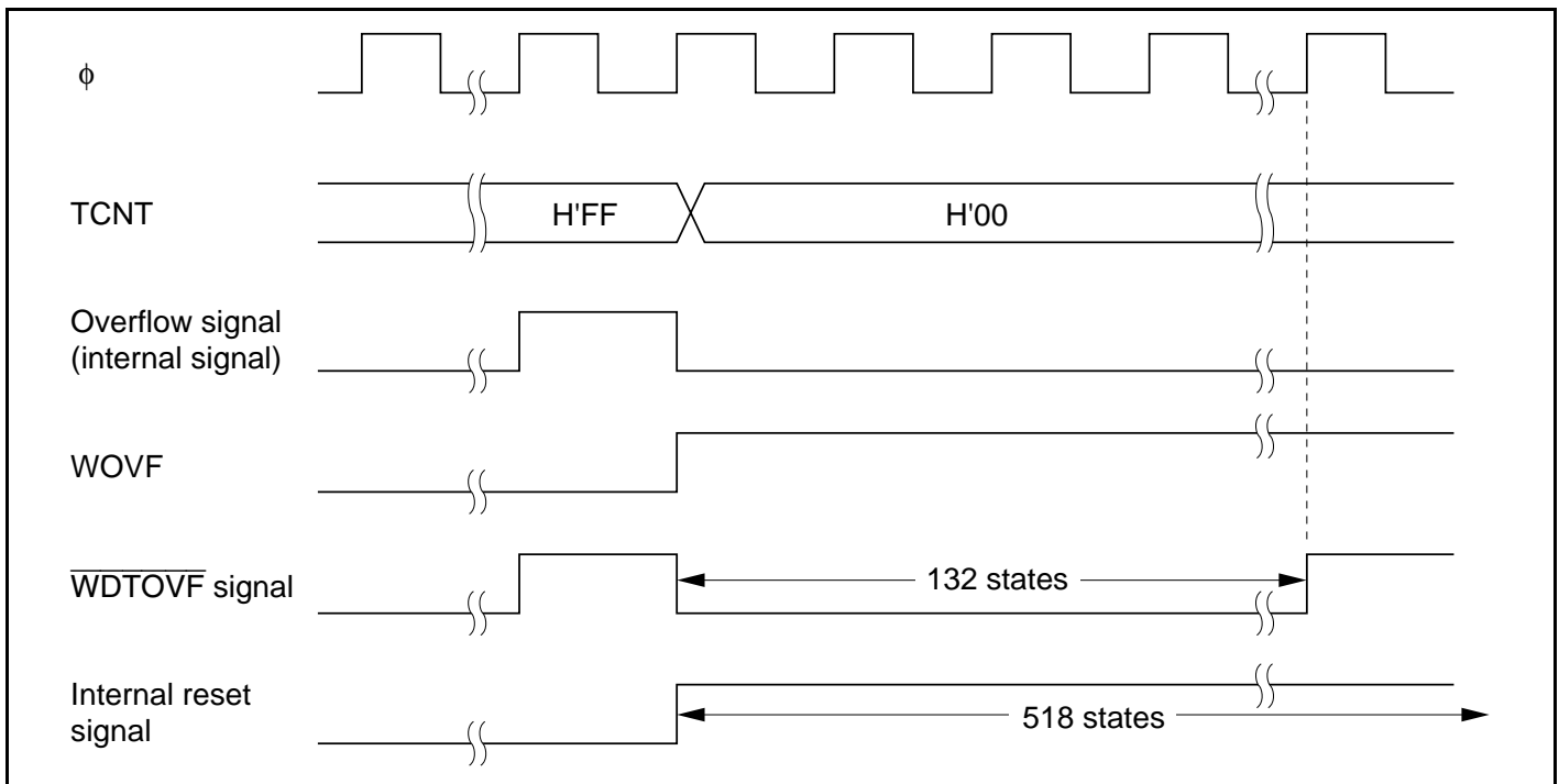
Figure 12.7 Timing of Setting of WOVF
