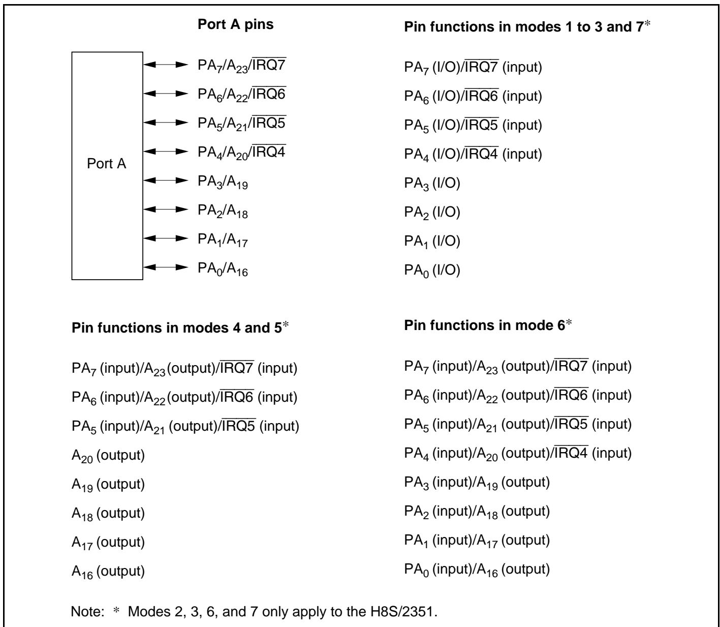
Figure 9.7 Port A Pin Functions
