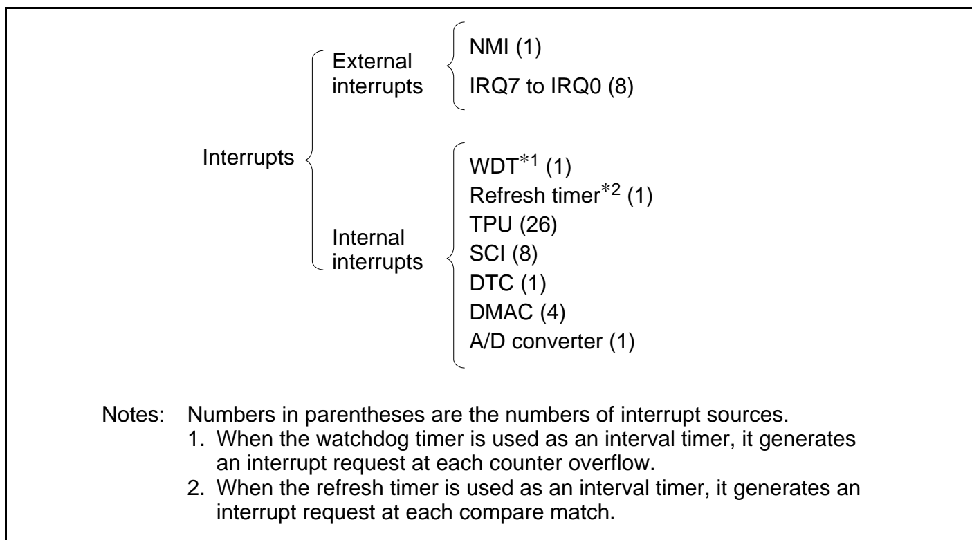
Figure 4.4 Interrupt Sources and Number of Interrupts
