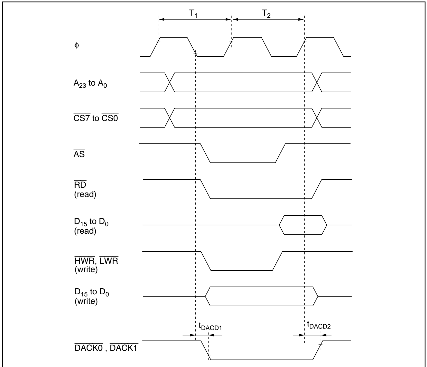
Figure 21.18 DMAC Single Address Transfer Timing (Two-State Access)
