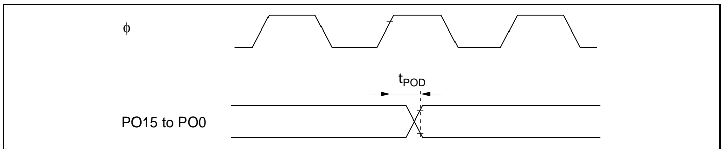
Figure 21.23 PPG Output Timing
