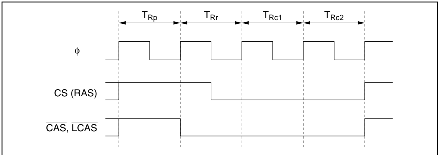
Figure 6.25 CBR Refresh Timing
