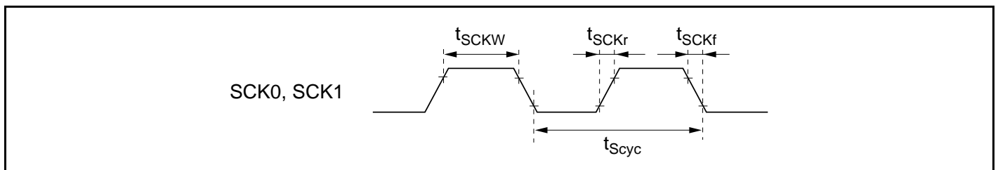
Figure 21.27 SCK Clock Input Timing
