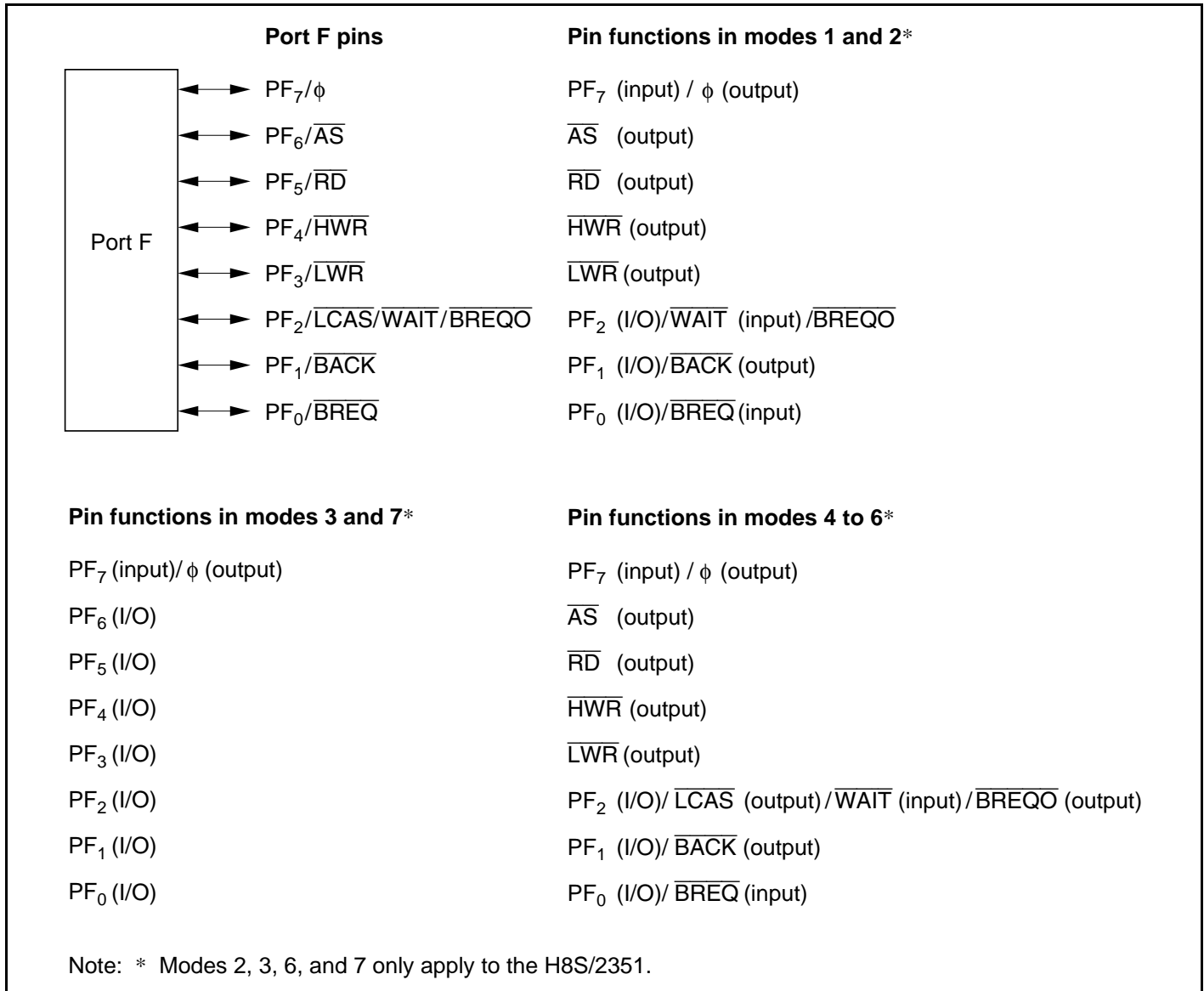
Figure 9.25 Port F Pin Functions
