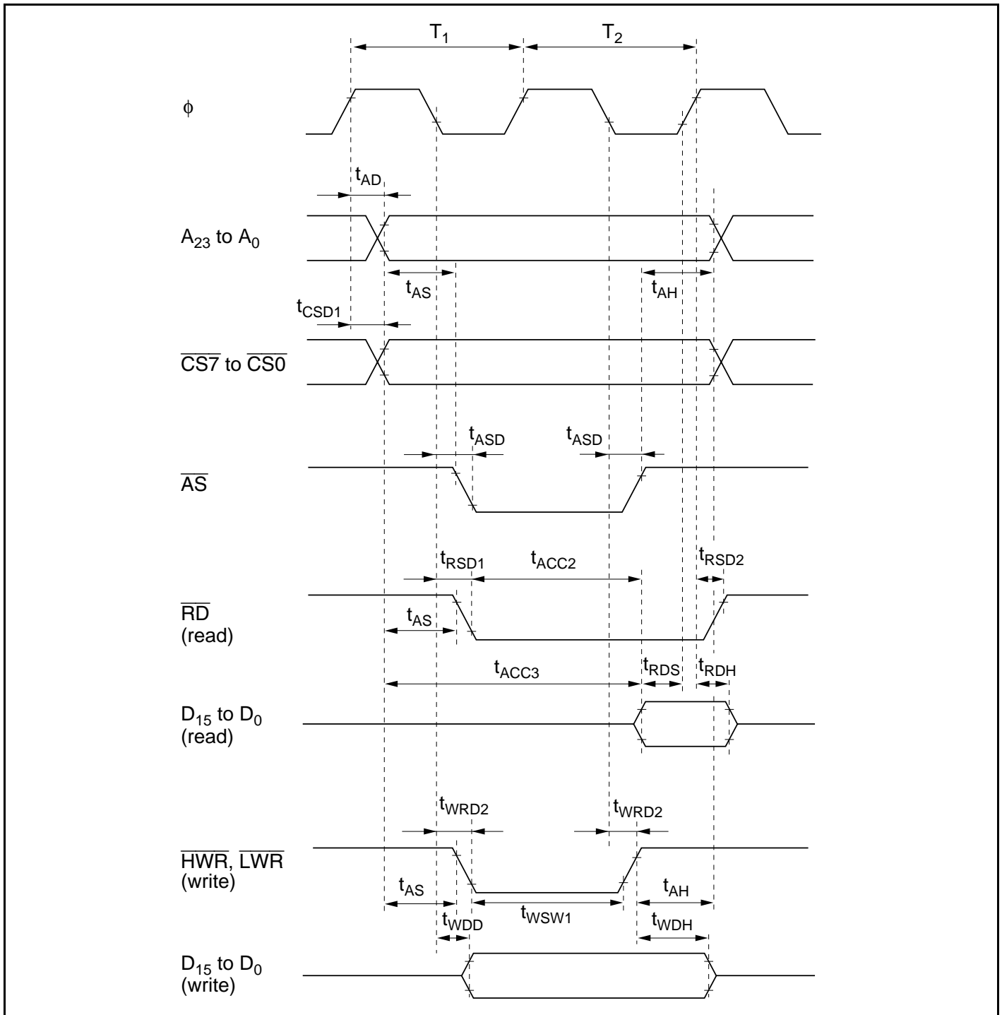
Figure 21.8 Basic Bus Timing (Two-State Access)
