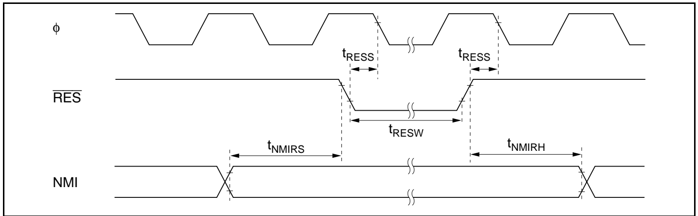
Figure 21.6 Reset Input Timing
