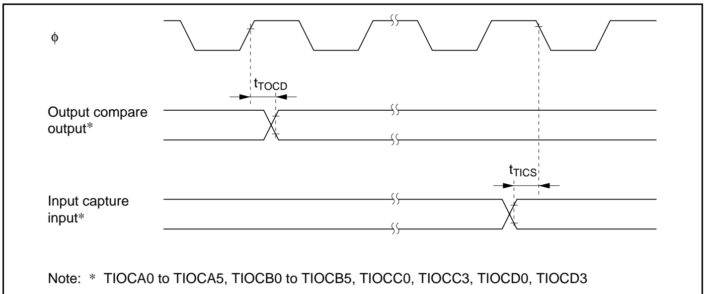
Figure 21.24 TPU Input/Output Timing
