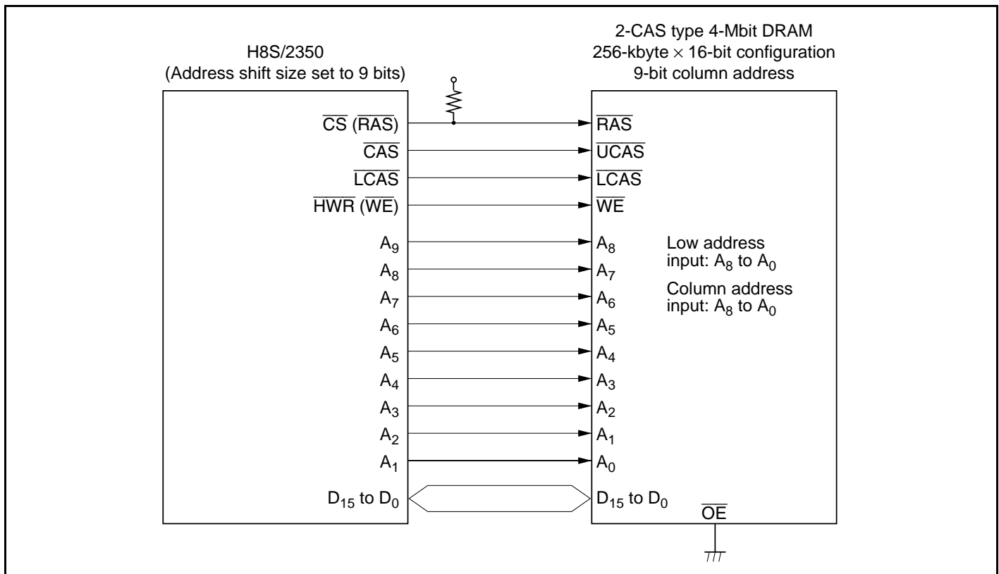
Figure 6.19 Example of 2-CAS System Connection
