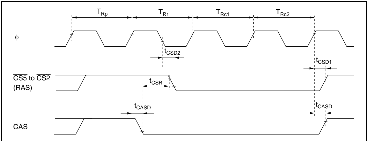
Figure 21.12 CAS-Before-RAS Refresh Timing
