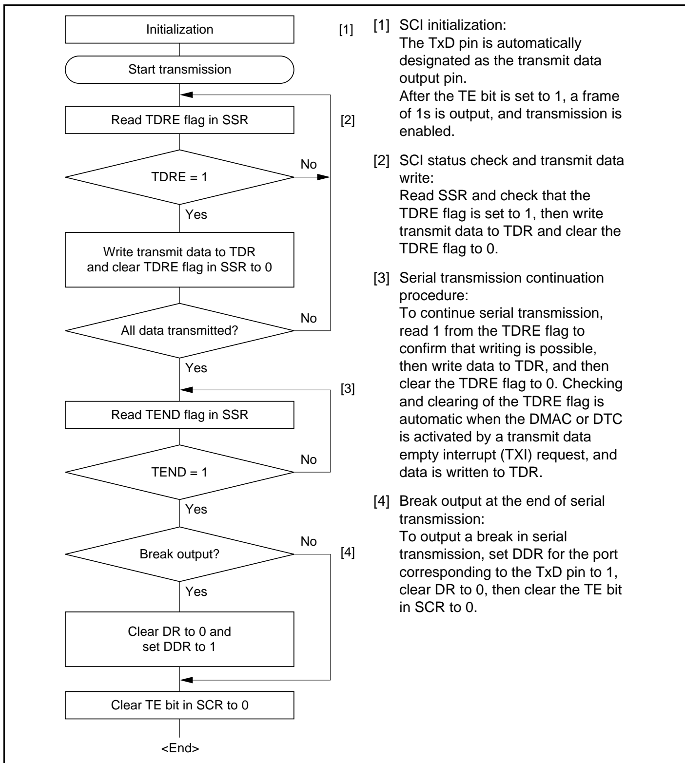
Figure 13.5 Sample Serial Transmission Flowchart
