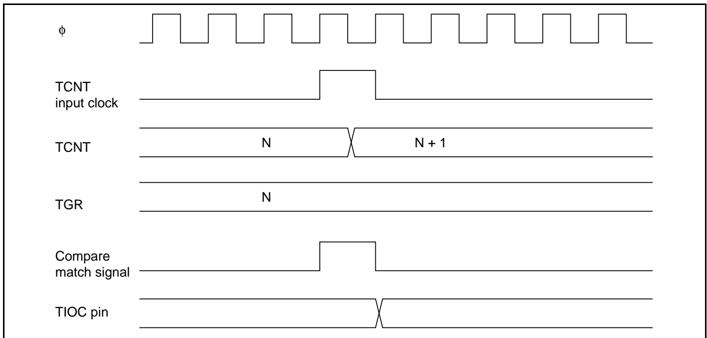
Figure 10.36 Output Compare Output Timing
