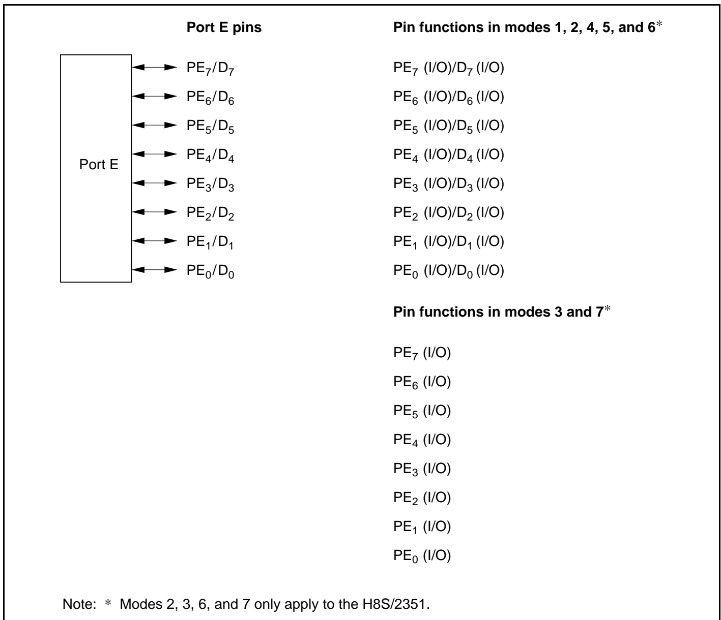
Figure 9.22 Port E Pin Functions
