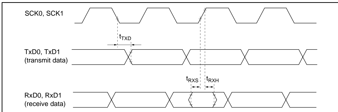
Figure 21.28 SCI Input/Output Timing (Clock Synchronous Mode)
