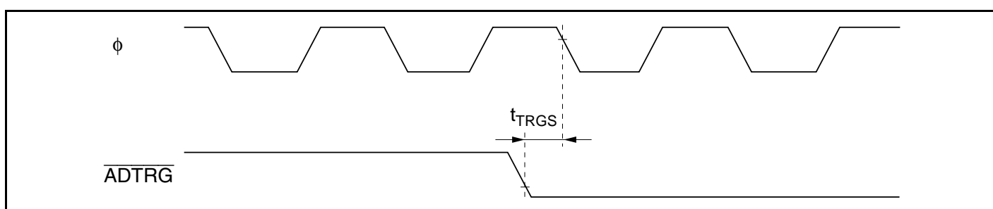
Figure 21.29 A/D Converter External Trigger Input Timing
