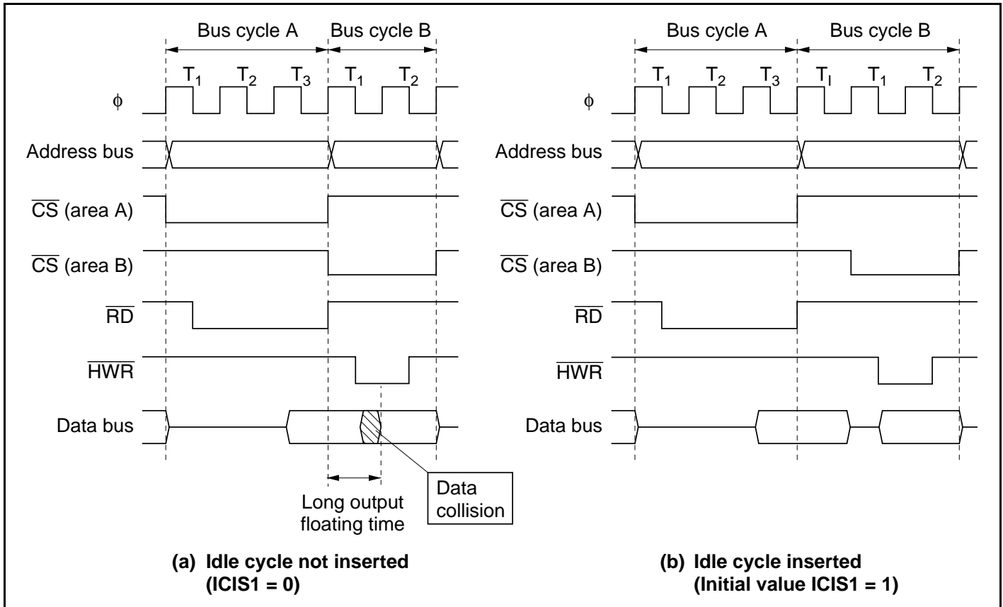
Figure 6.32 Example of Idle Cycle Operation (2)
