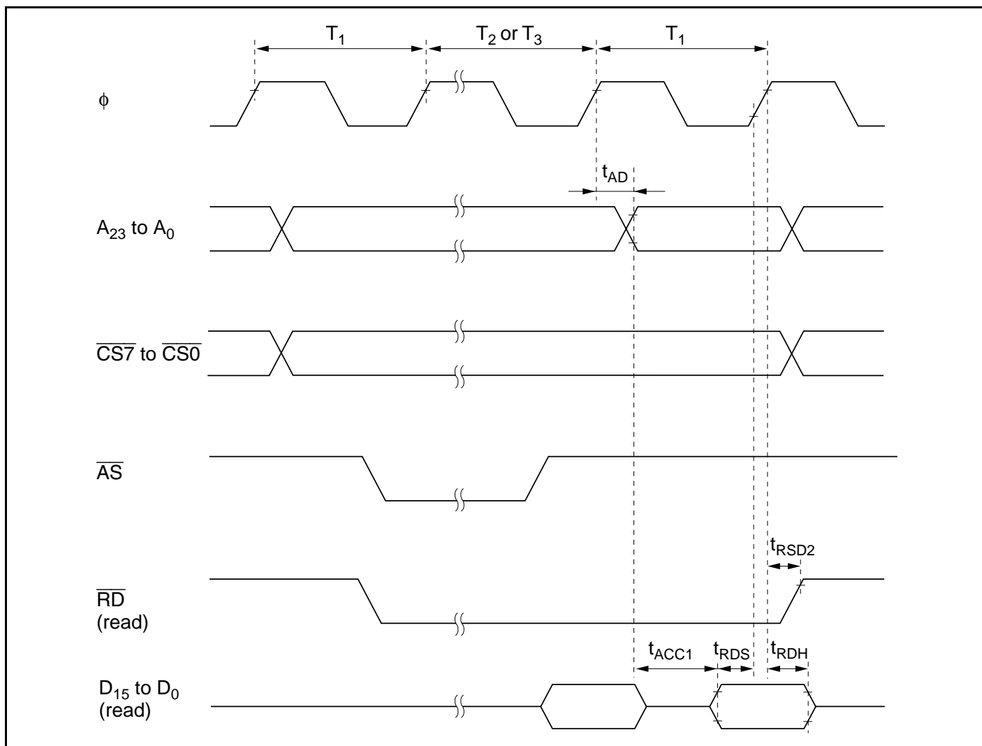
Figure 21.15 Burst ROM Access Timing (One-State Access)
