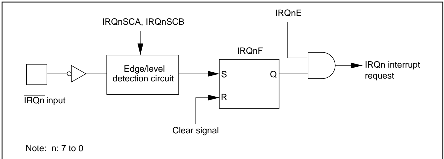
Figure 5.2 Block Diagram of Interrupts IRQ7 to IRQ0
