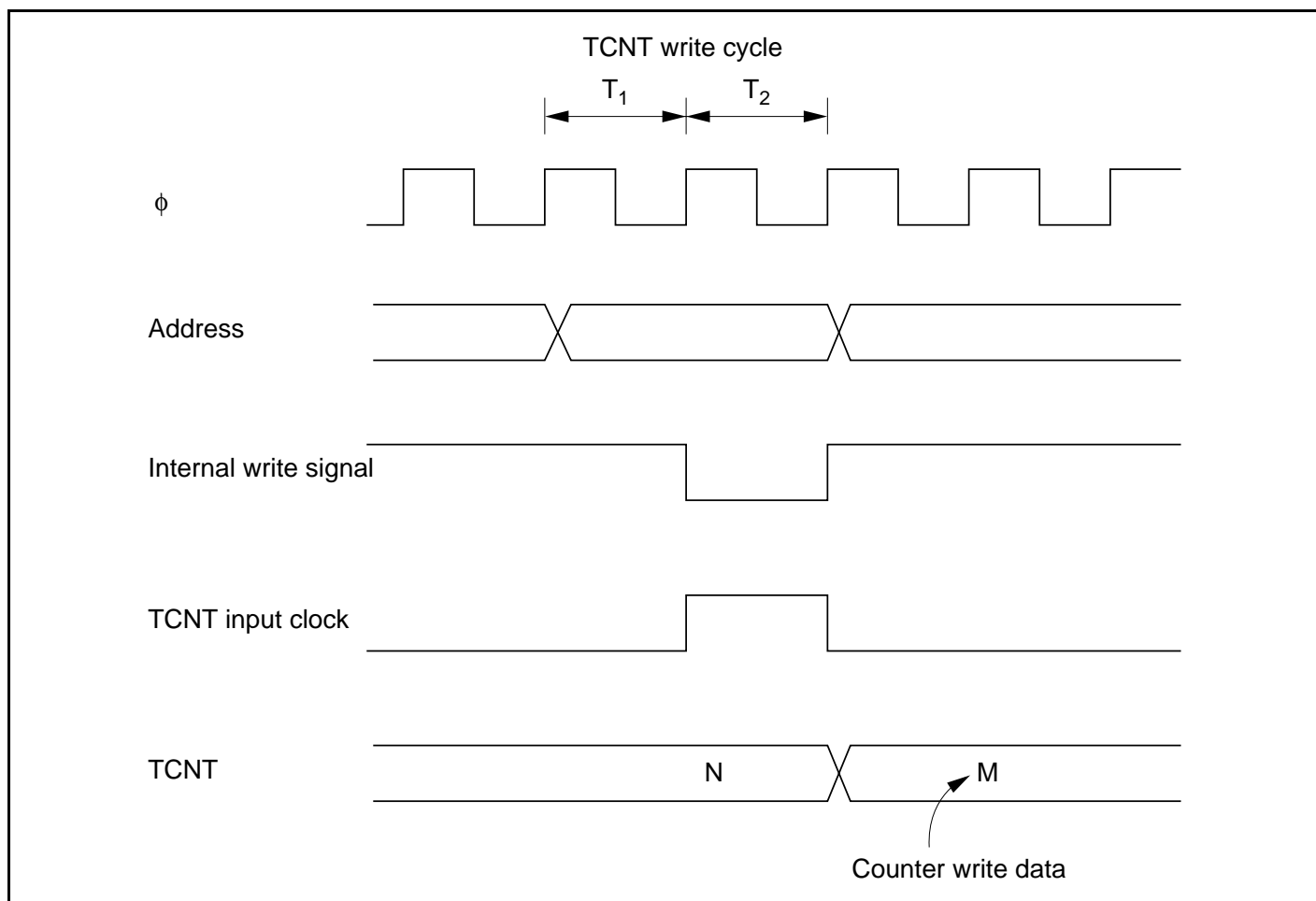
Figure 12.8 Contention between TCNT Write and Increment
