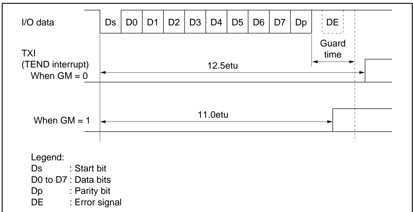
Figure 14.6 TEND Flag Generation Timing in Transmission Operation
