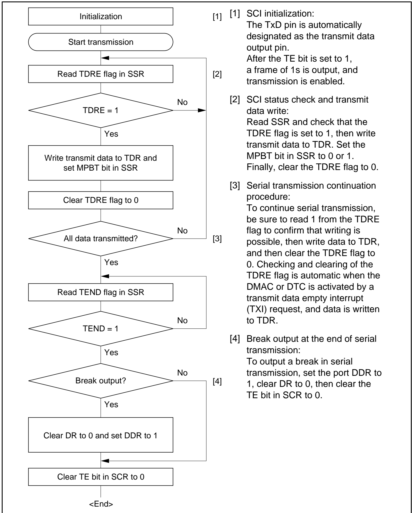
Figure 13.10 Sample Multiprocessor Serial Transmission Flowchart
