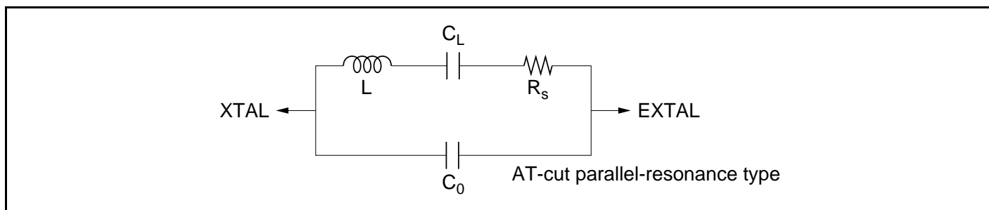
Figure 19.3 Crystal Resonator Equivalent Circuit
