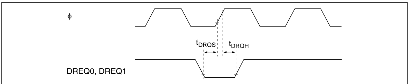
Figure 21.21 DMAC \overline{DREQ} Input Timing
