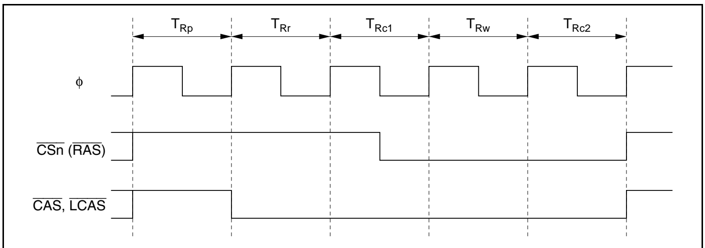
Figure 6.26 CBR Refresh Timing (When RCW = 1, RLW1 = 0, RLW0 = 1)
