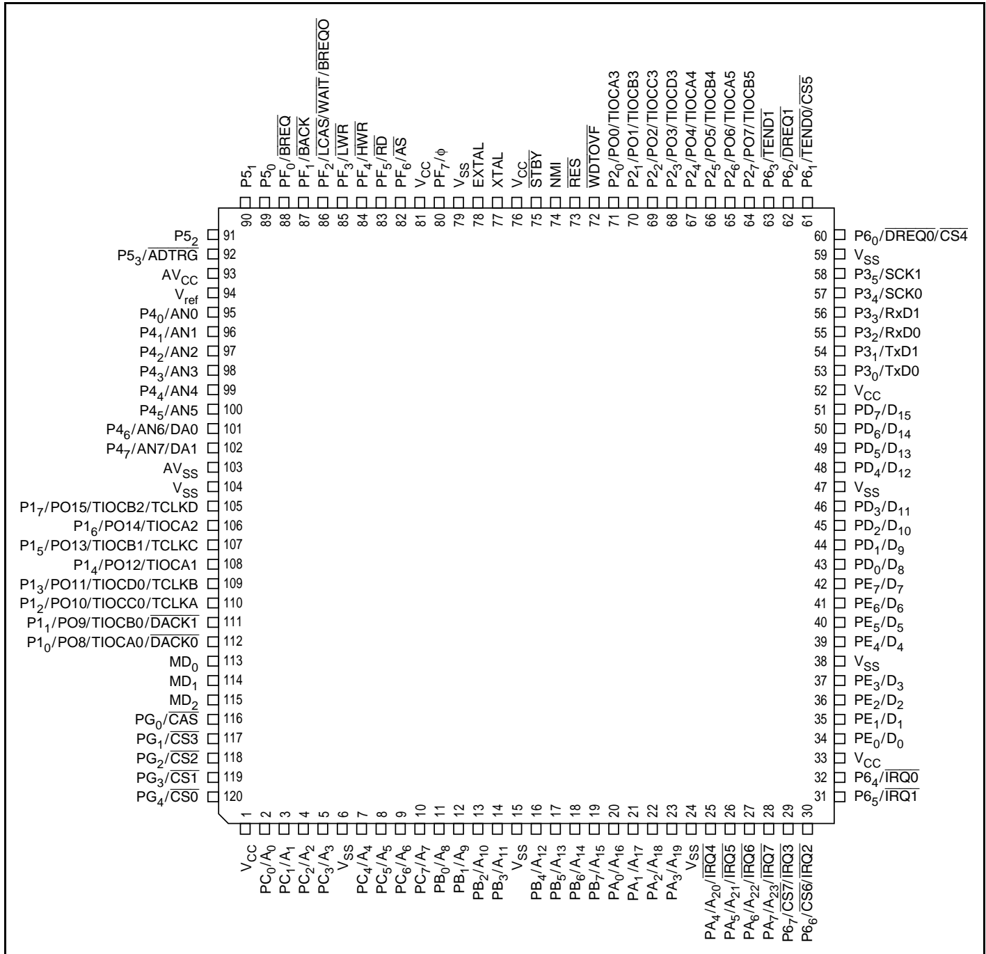
Figure 1.2 Pin Arrangement (TFP-120: Top View)
