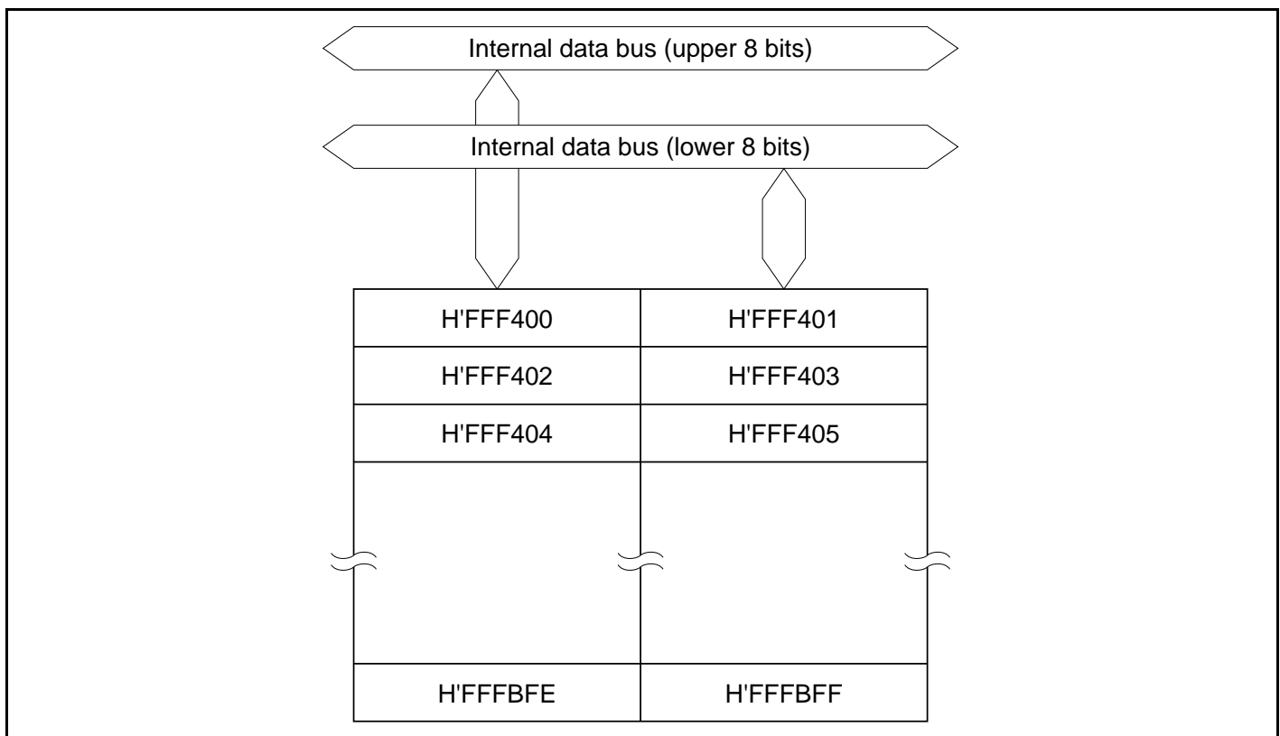
Figure 17.1 Block Diagram of RAM
