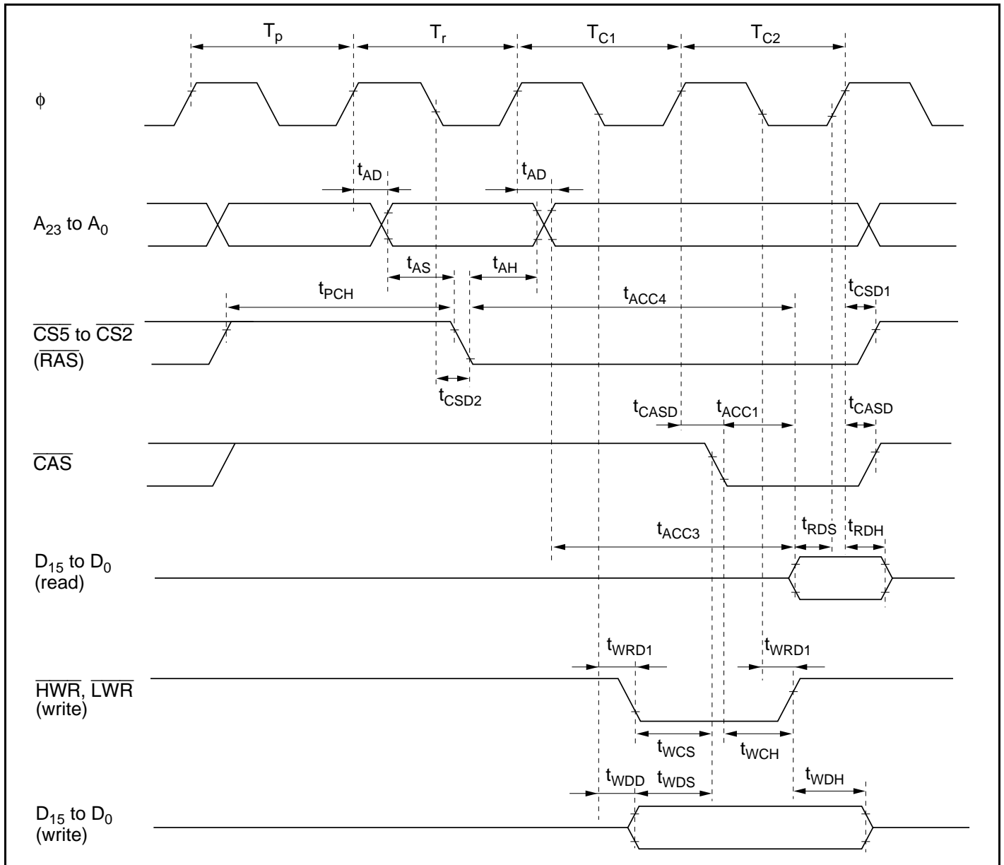
Figure 21.11 DRAM Bus Timing
