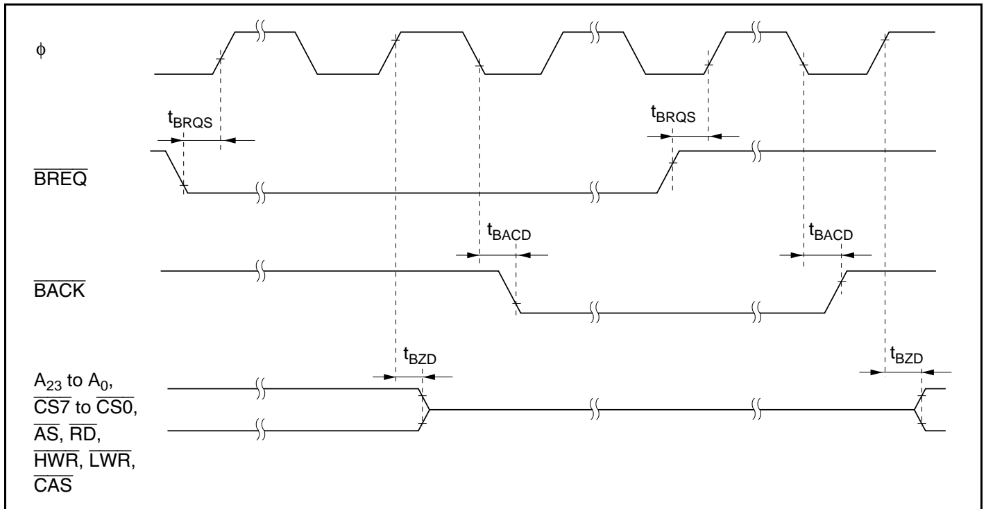
Figure 21.16 External Bus Release Timing
