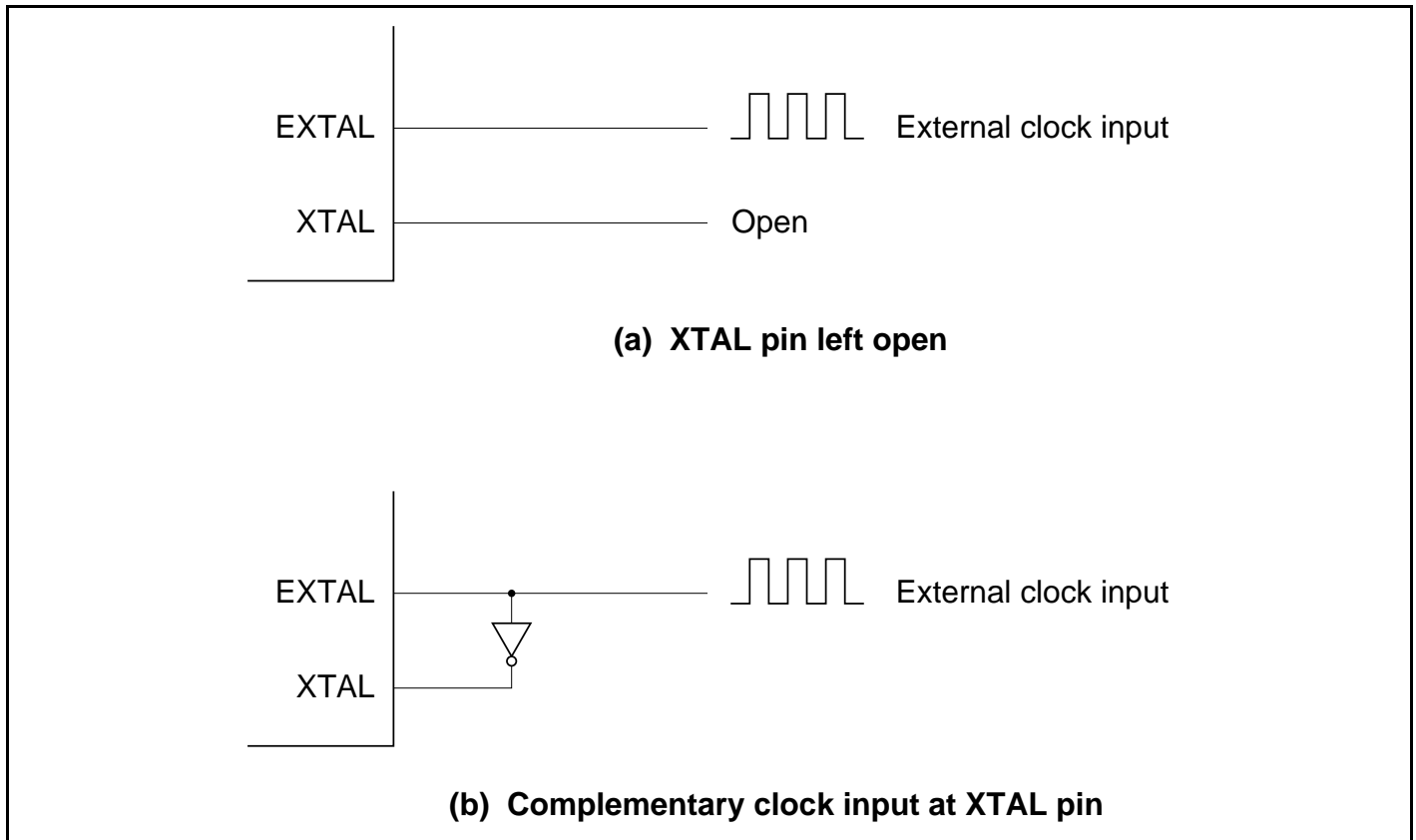
Figure 19.5 External Clock Input (Examples)
