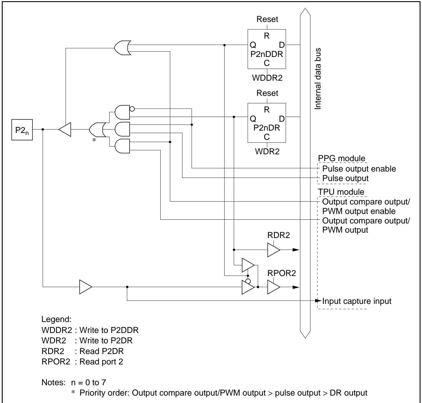
Figure C.2 Port 2 Block Diagram (Pin P2 n )
