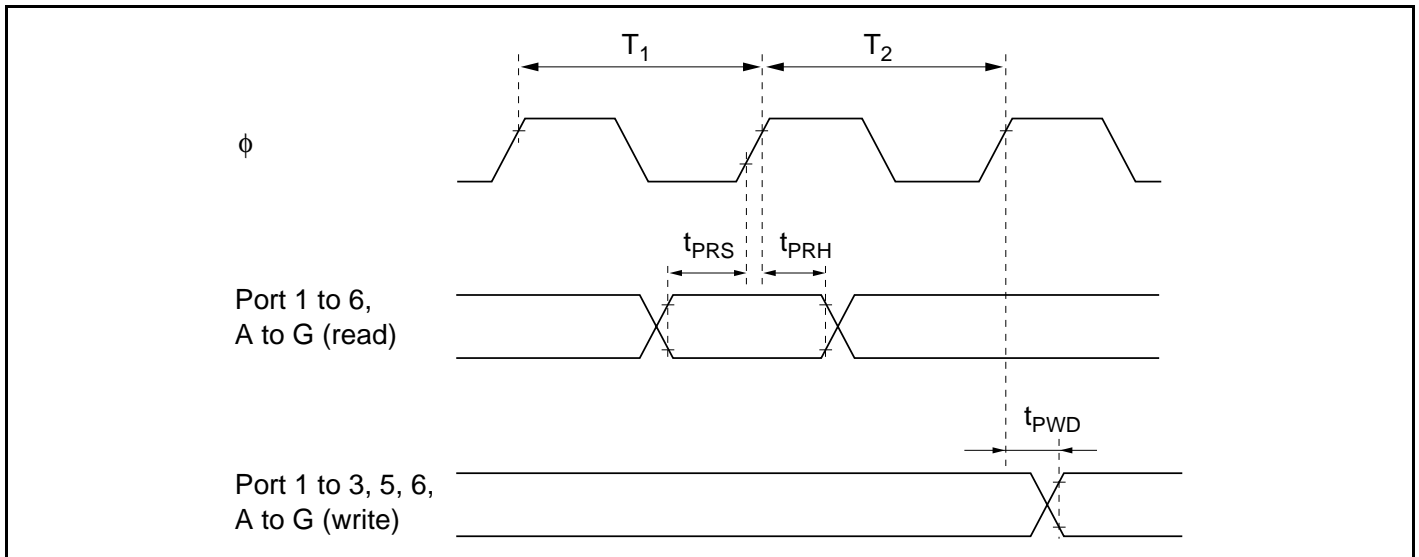
Figure 21.22 I/O Port Input/Output Timing
