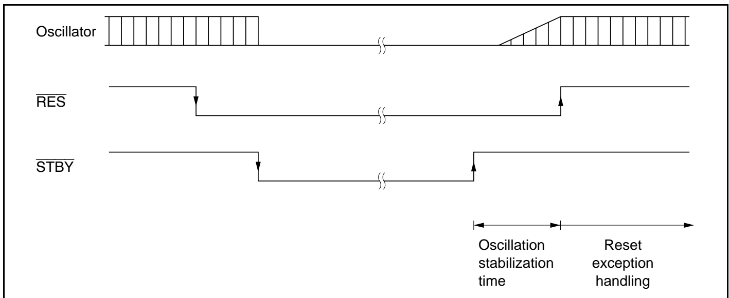
Figure 20.3 Hardware Standby Mode Timing (Example)
