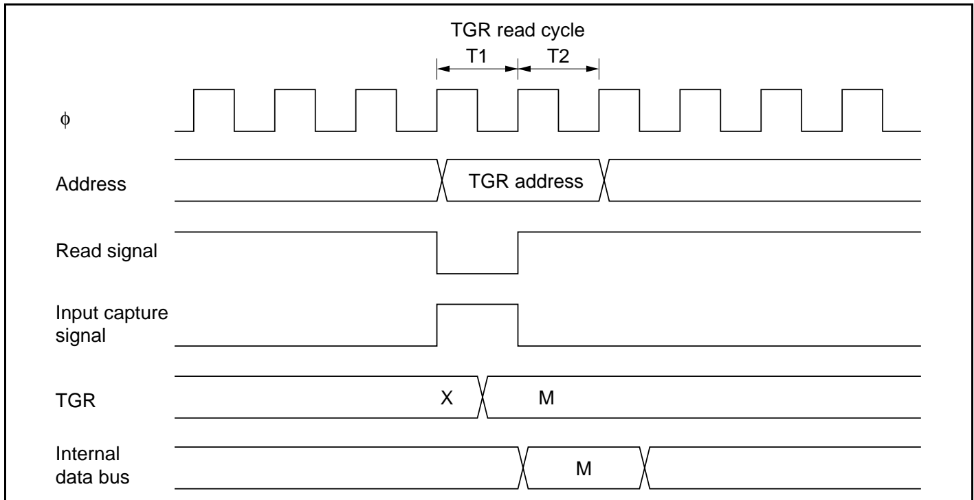
Figure 10.53 Contention between TGR Read and Input Capture
