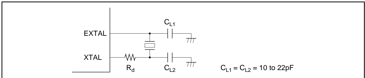
Figure 19.2 Connection of Crystal Resonator (Example)
