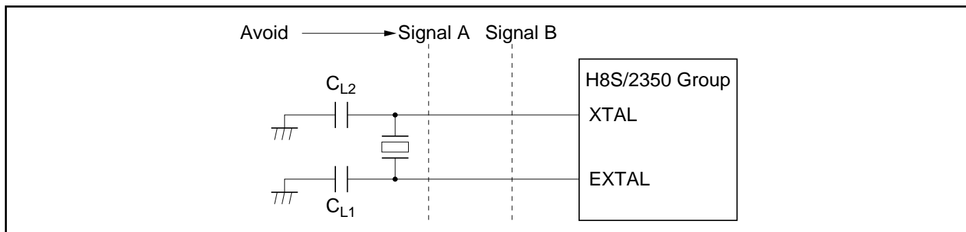
Figure 19.4 Example of Incorrect Board Design
