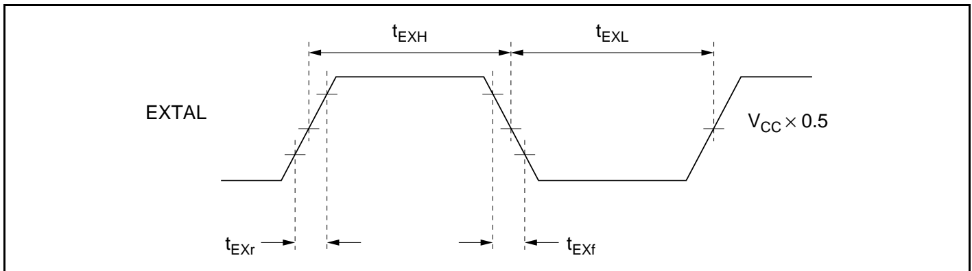
Figure 19.6 External Clock Input Timing
