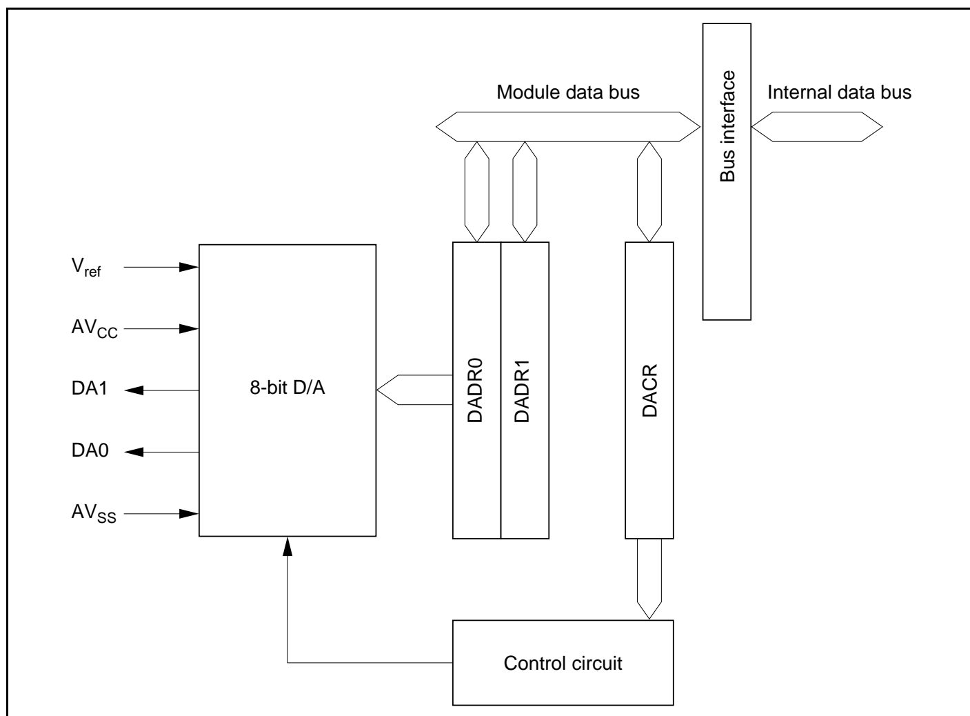
Figure 16.1 Block Diagram of D/A Converter
