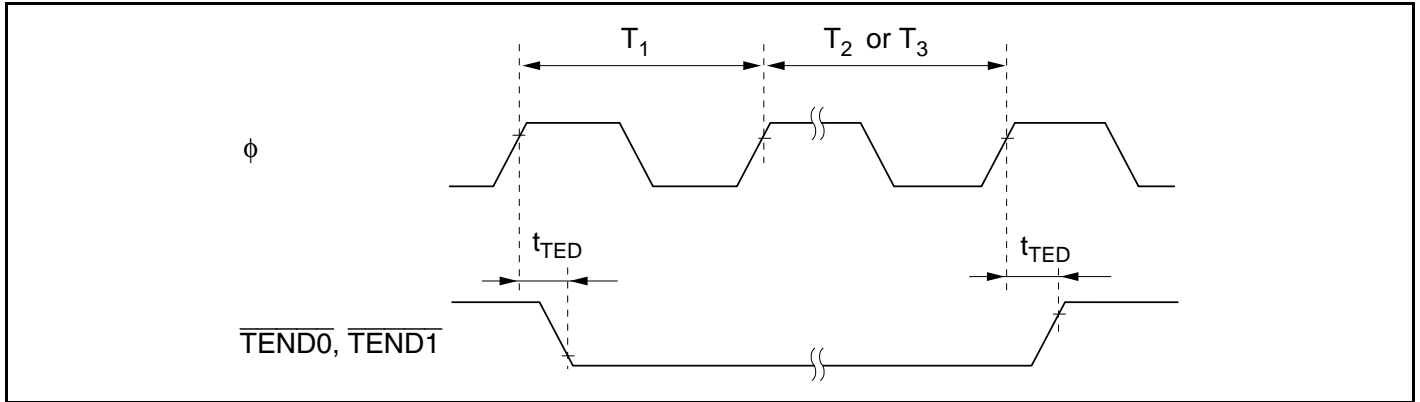
Figure 21.20 DMAC \overline{TEND} Output Timing
