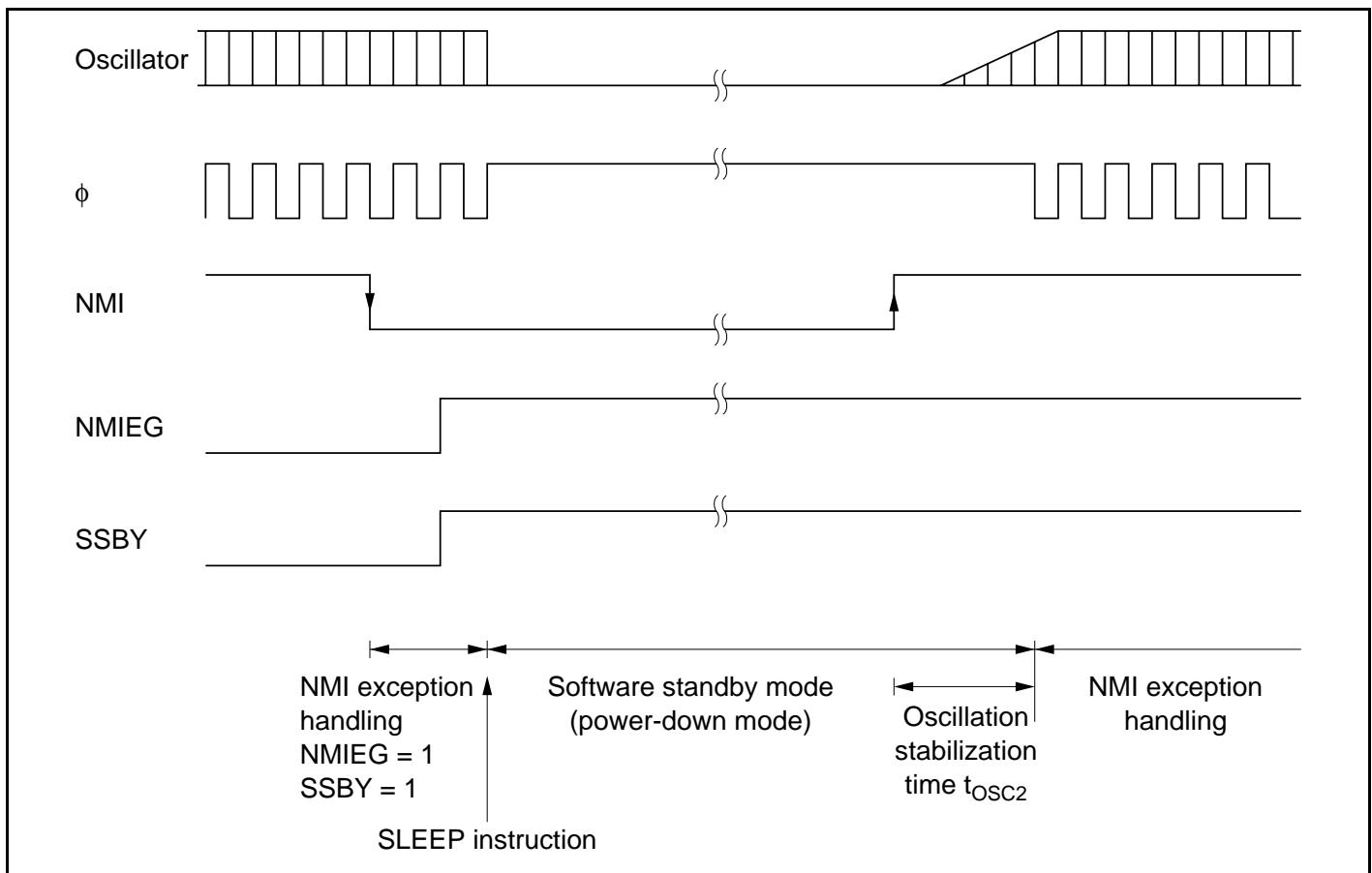
Figure 20.2 Software Standby Mode Application Example
