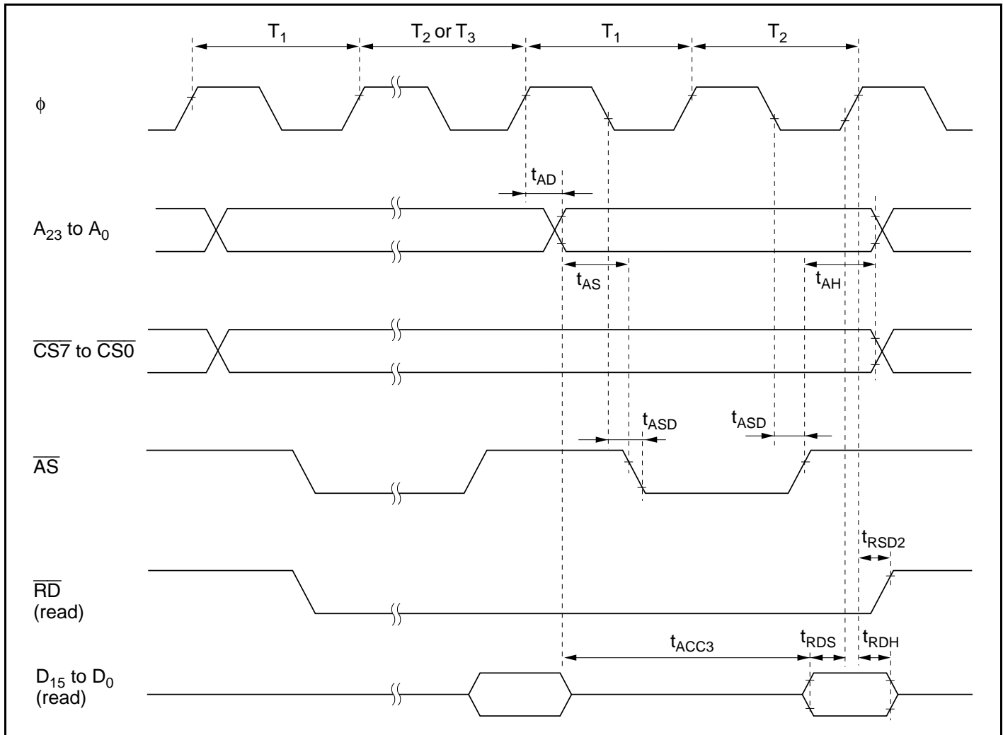
Figure 21.14 Burst ROM Access Timing (Two-State Access)
