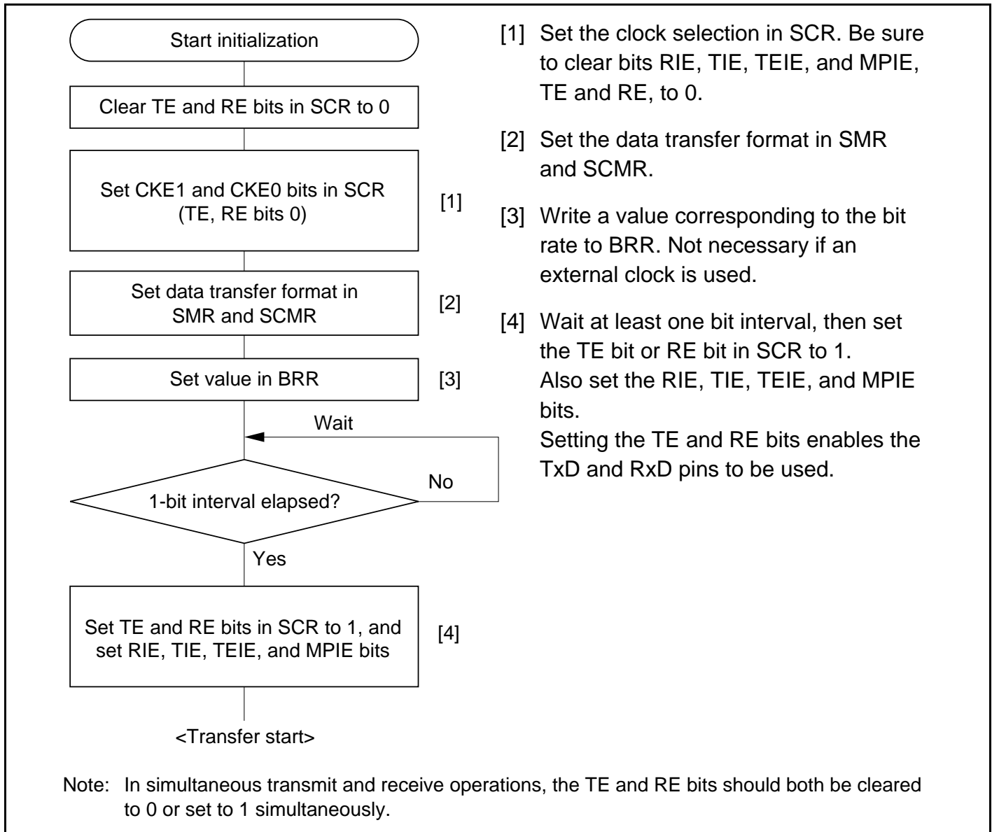
Figure 13.15 Sample SCI Initialization Flowchart
