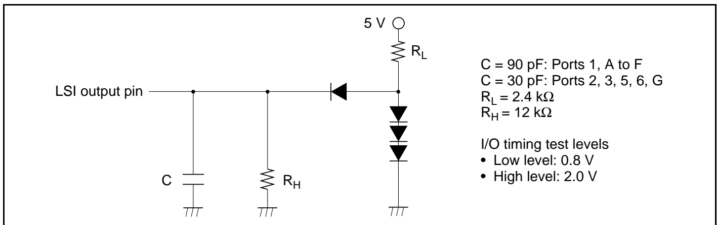
Figure 21.3 Output Load Circuit
