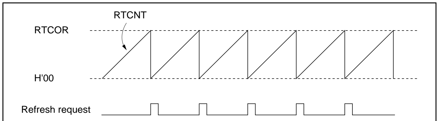
Figure 6.23 RTCNT Operation
