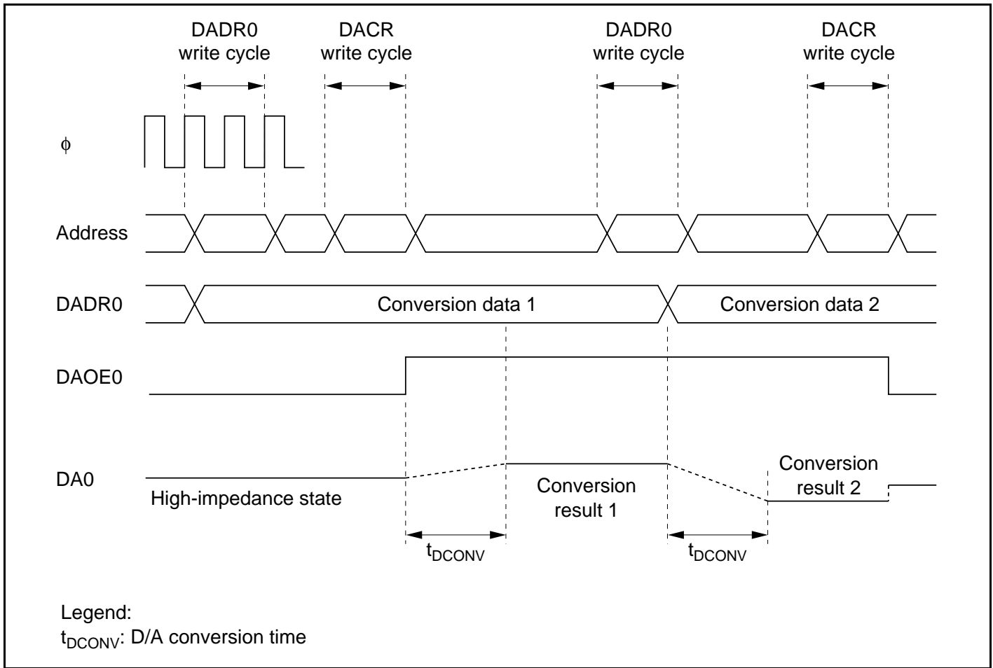
Figure 16.2 Example of D/A Converter Operation
