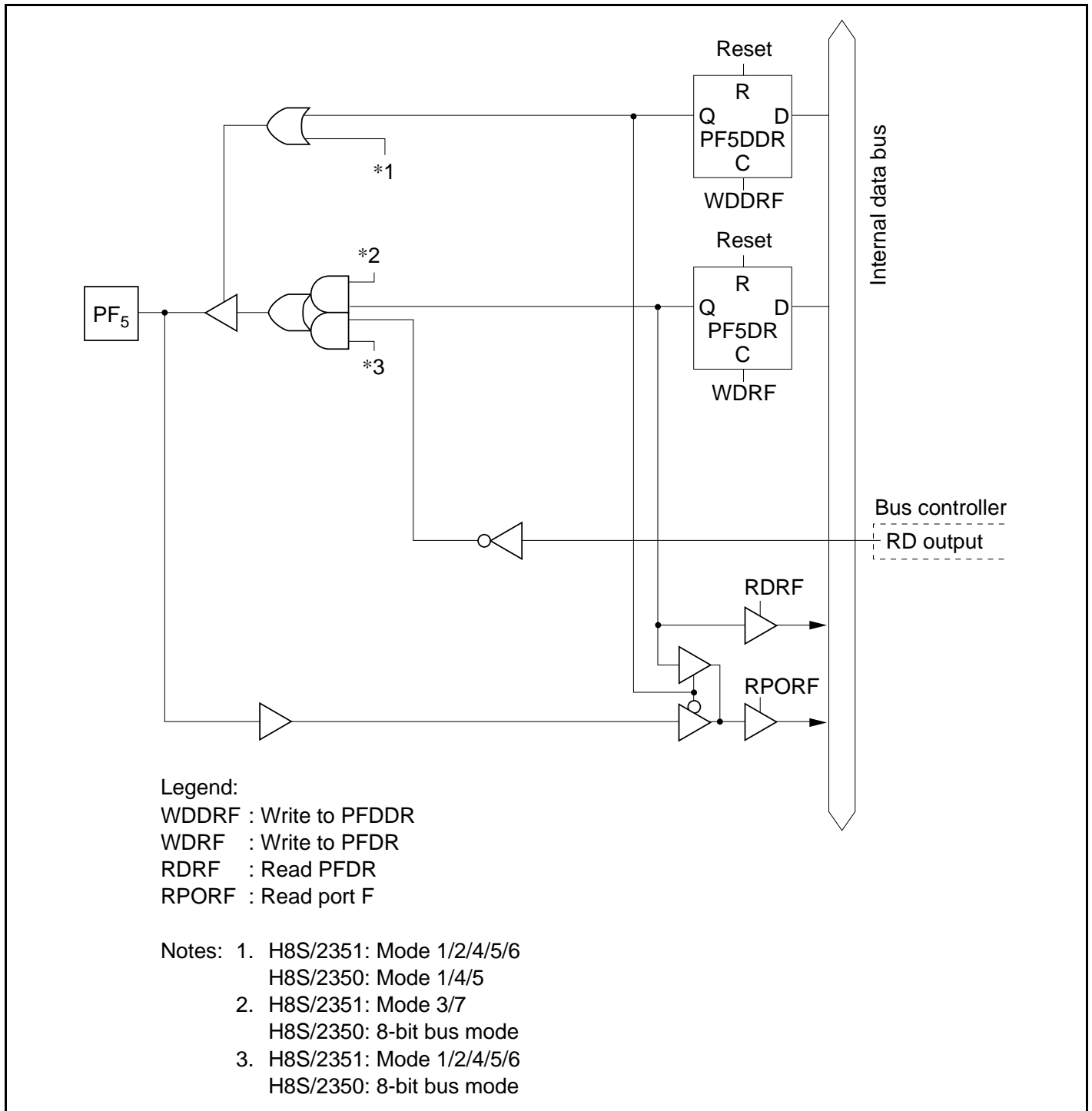
Figure C.12 (f) Port F Block Diagram (Pin PF 5 )
