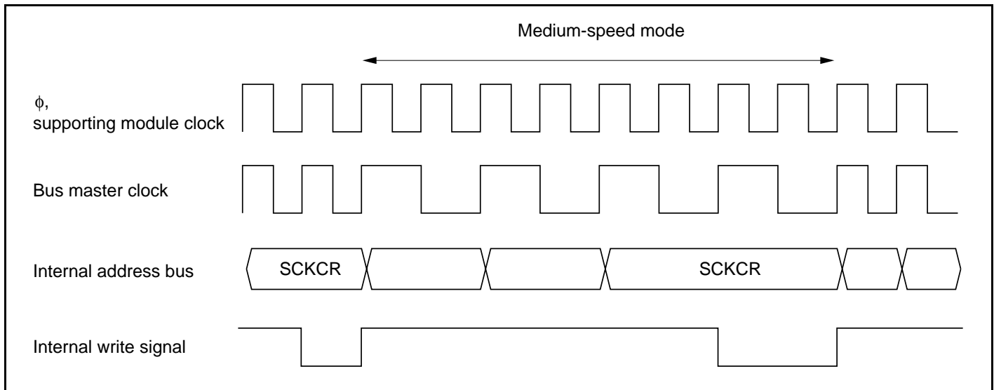
Figure 20.1 Medium-Speed Mode Transition and Clearance Timing
