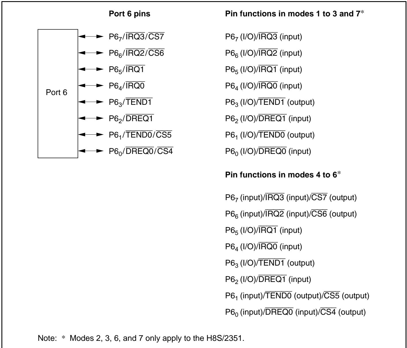
Figure 9.6 Port 6 Pin Functions
