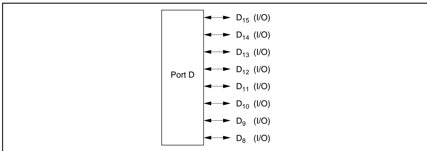
Figure 9.20 Port D Pin Functions (Modes 1, 2, and 4 to 6)
