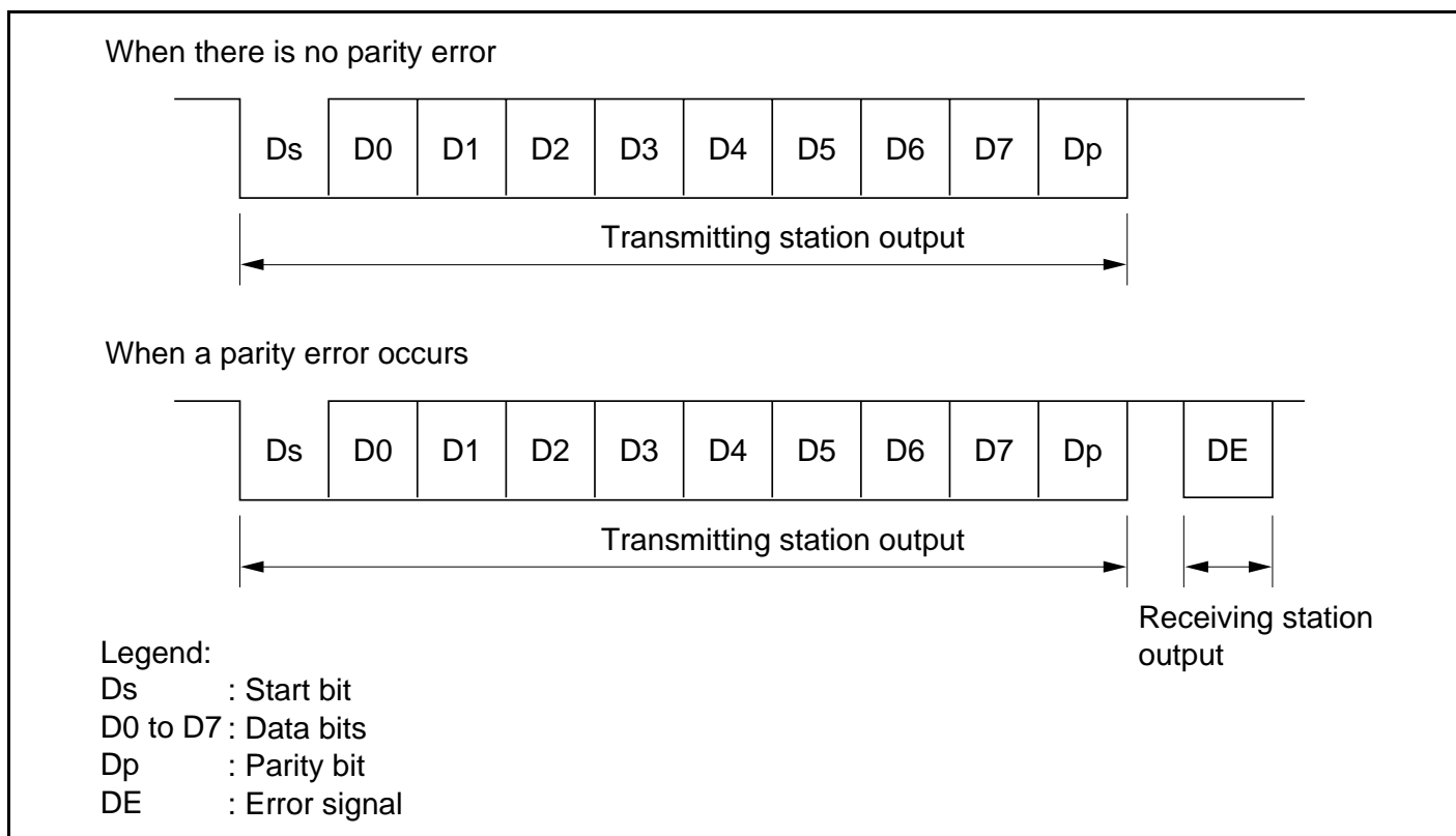
Figure 14.3 Smart Card Interface Data Format
