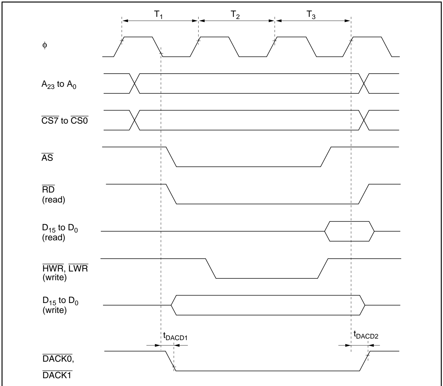
Figure 21.19 DMAC Single Address Transfer Timing (Three-State Access)
