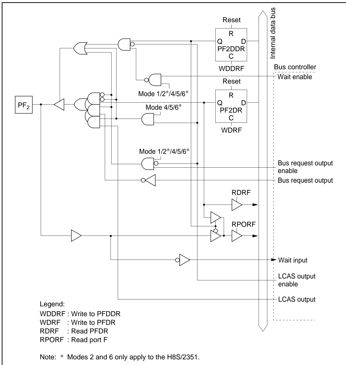
Figure C.12 (c) Port F Block Diagram (Pin PF 2 )
