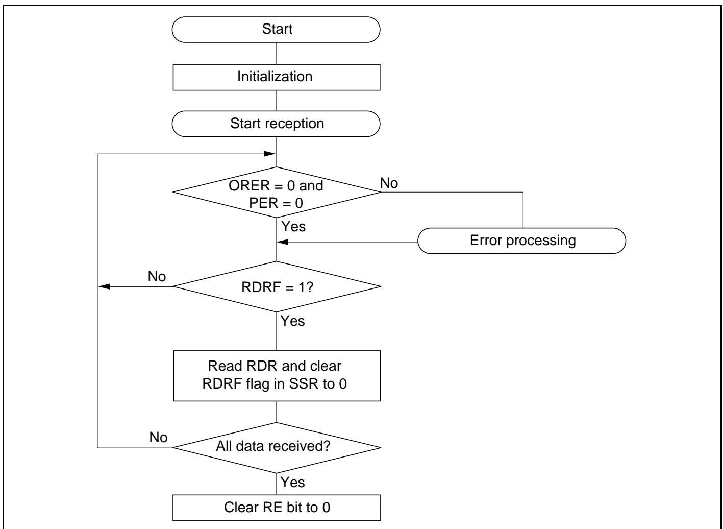
Figure 14.7 Example of Reception Processing Flow
