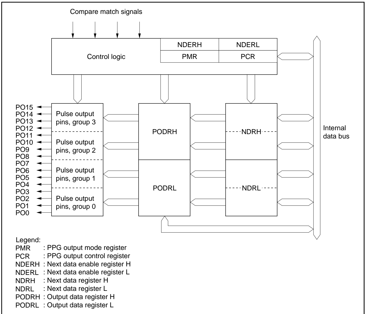
Figure 11.1 Block Diagram of PPG
