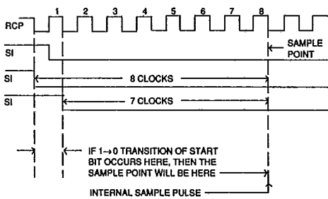
FIG. 7 TRUE RECEIVER CENTER SAMPLING
