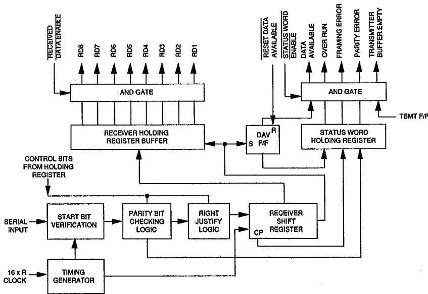
FIG. 25 RECEIVER BLOCK DIAGRAM
