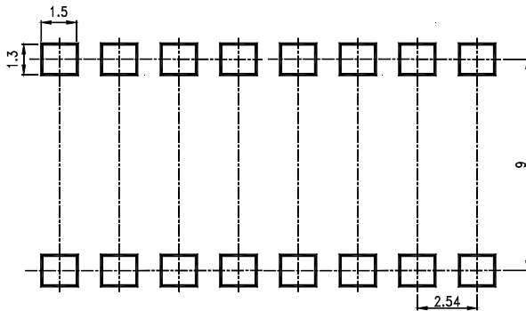
16 PIN
