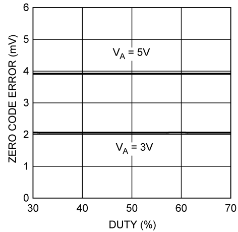
Zero Code Error vs. Clock Duty Cycle
