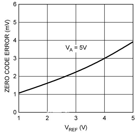
Zero Code Error vs. V_{REFIN}
