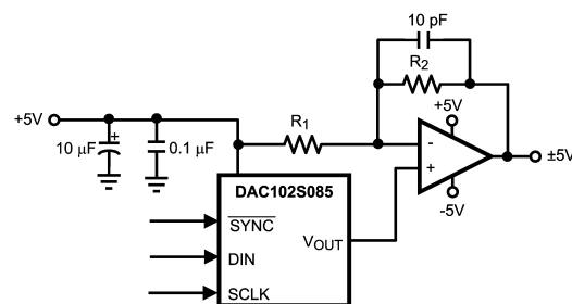
FIGURE 9. Bipolar Operation
