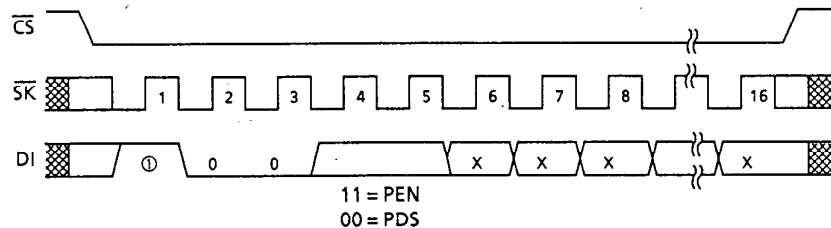
Figure 7 PEN/PDS Timing
