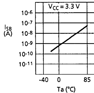
1.8 Standby current consumption I_{SB} — Ambient temperature T_a
