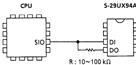
Figure 8 3-wire interface
