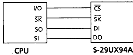
Figure 9 Connectin Example
