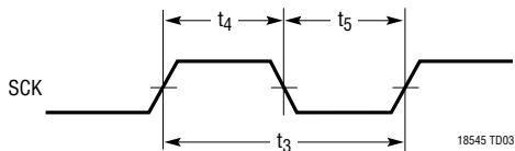
t_3, t_4, t_5 (SCK Timing)
