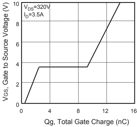
Figure 7. Gate Charge
