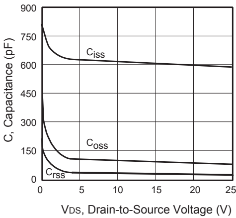
Figure 3. Capacitance
