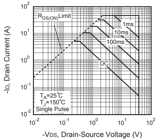
Figure 16. Maximum Safe Operating Area
