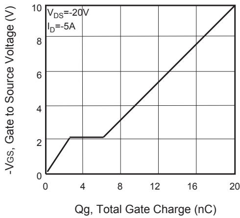
Figure 15. Gate Charge
