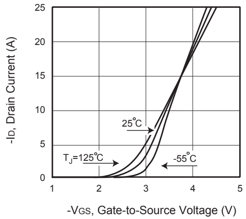
Figure 8. Transfer Characteristics
