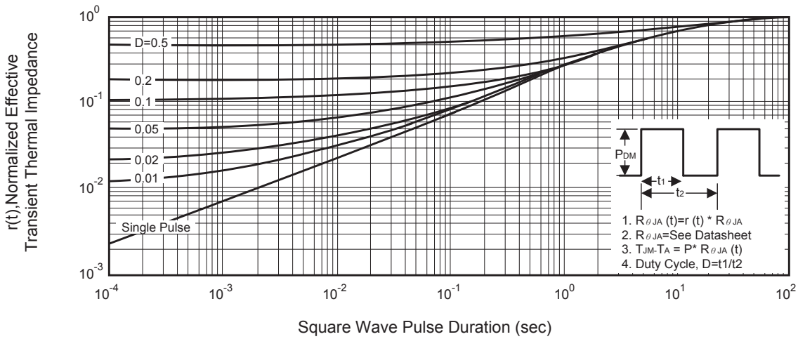
Figure 19. Normalized Thermal Transient Impedance Curve
