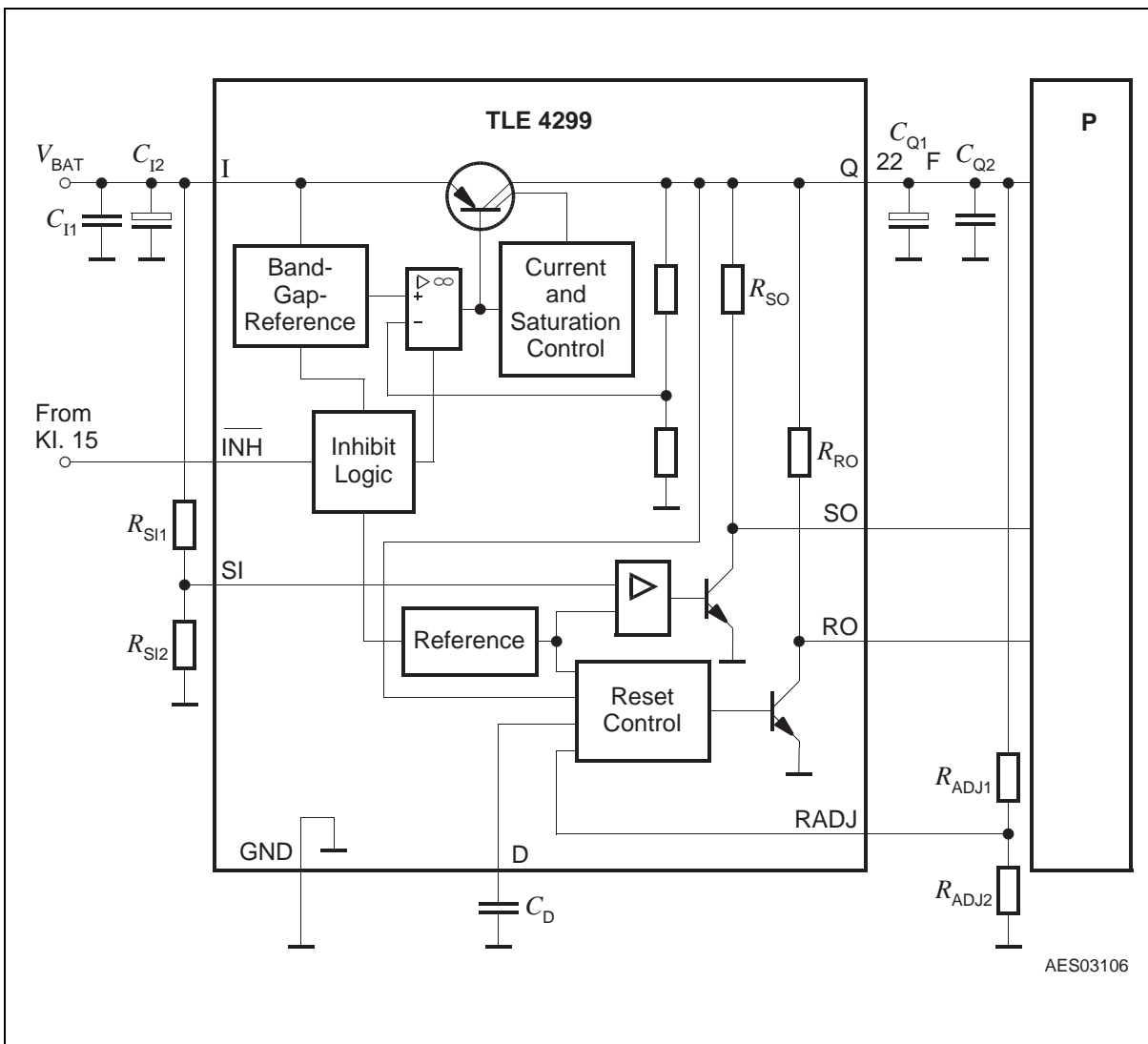
Figure 7 Application Diagram with Inhibit Function TLE4299 GMV33
