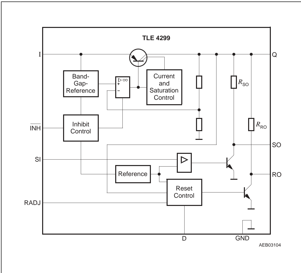
Figure 2 Block Diagram TLE 4299 GMV33
