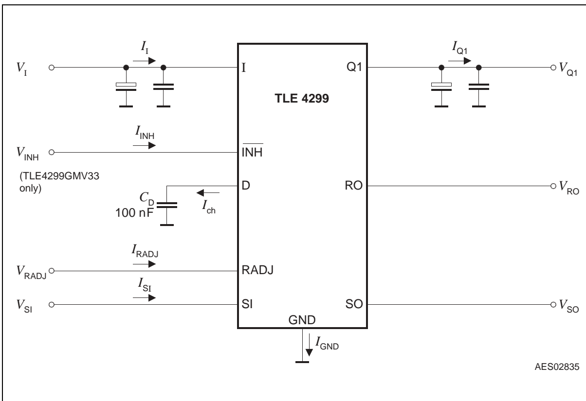
Figure 5 Measurement Circuit
