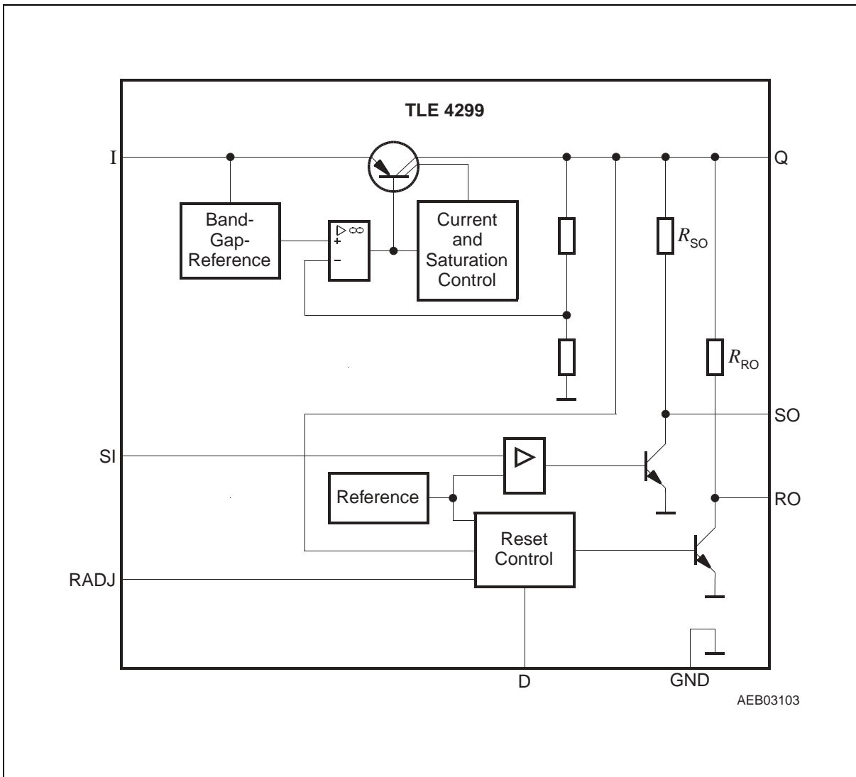
Figure 1 Block Diagram TLE 4299 GV33
