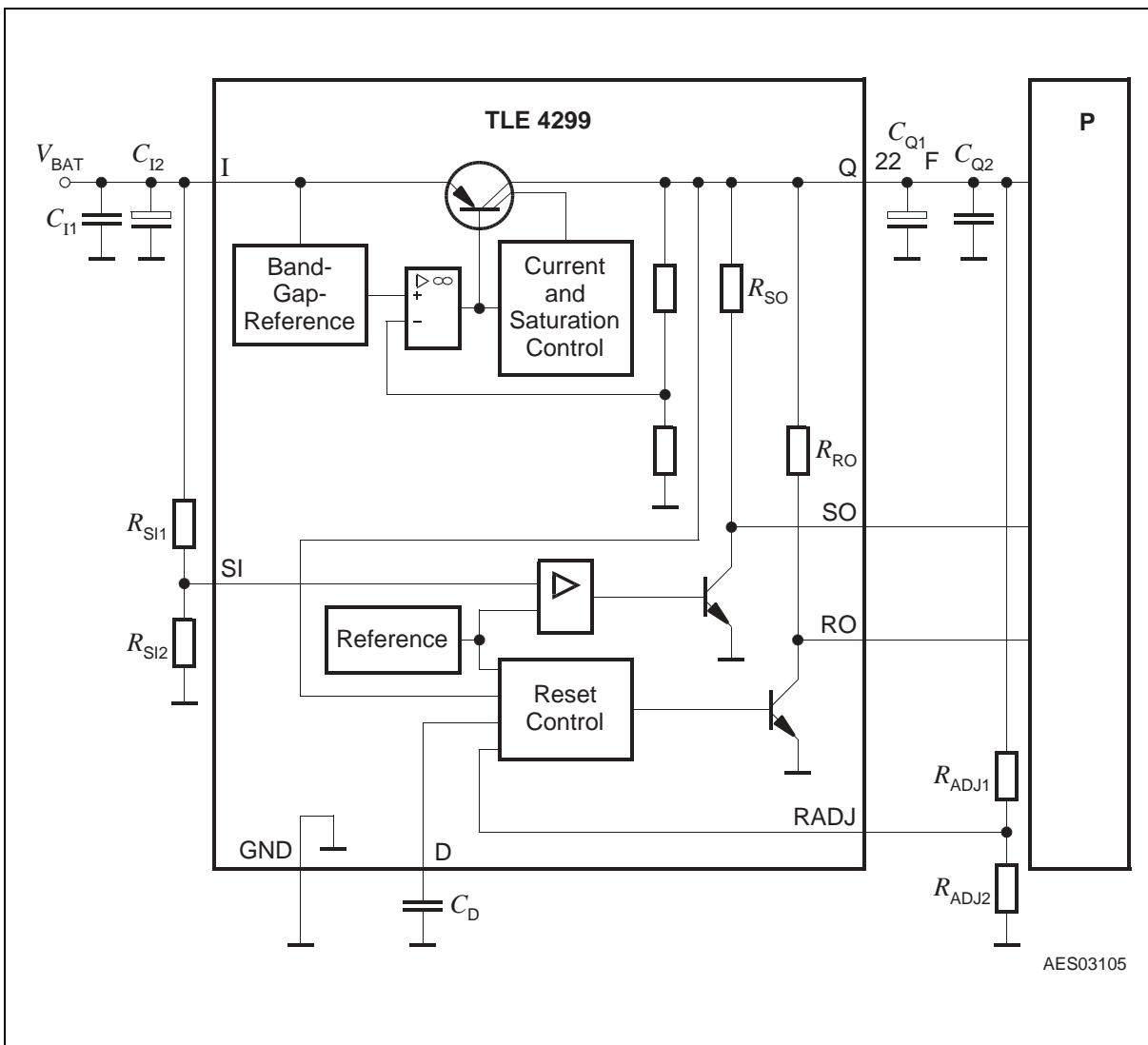
Figure 6 Application Diagram TLE 4299 GV33
