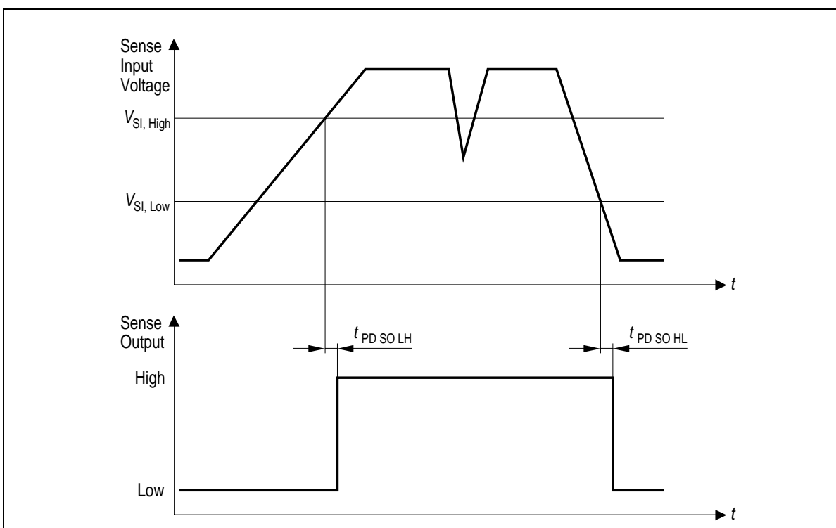
Figure 9 Sense Timing Diagram
