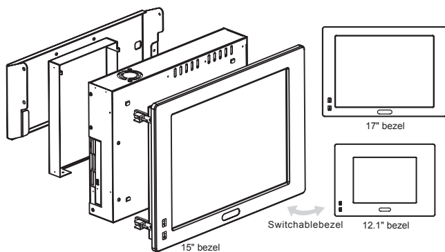
12.1" / 15" / 17" Modularizing View
