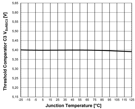
Figure 42 Threshold Comparator C3 V_{SoftSC3}
