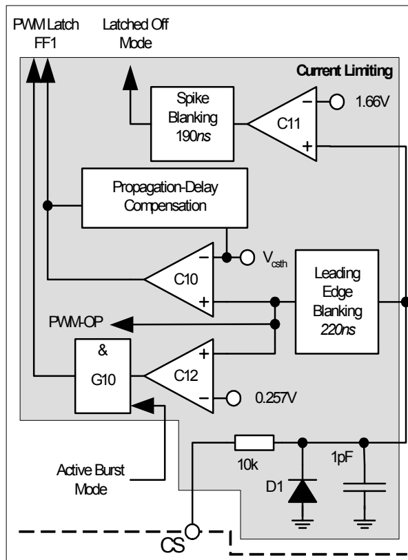
Figure 10 Current Limiting
