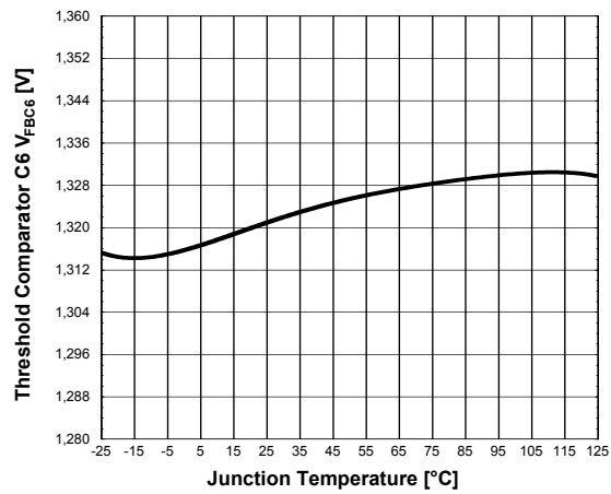
Figure 43 Threshold Comparator C6 V_{FBC6}
