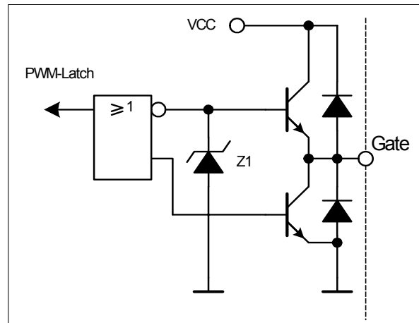
Figure 8 Gate Driver
