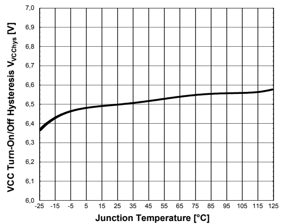
Figure 32 VCC Turn-On/Off Hysteresis V_{VCChys}
