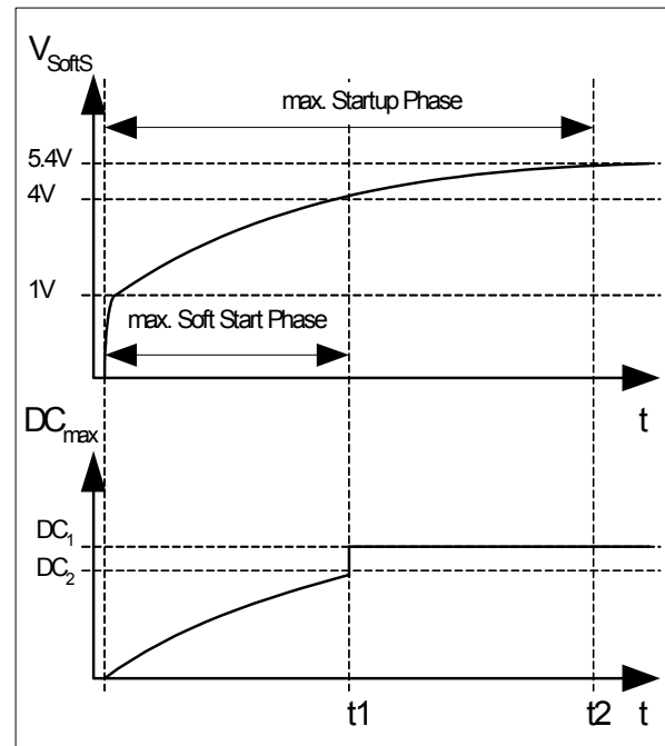
Figure 6 Startup Phase
