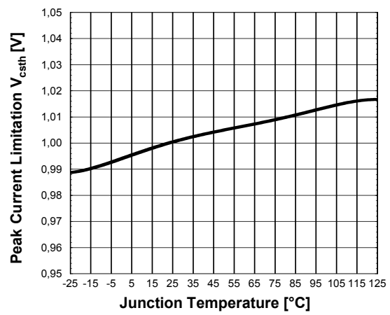
Figure 48 Peak Current Limitation V_{csth}
