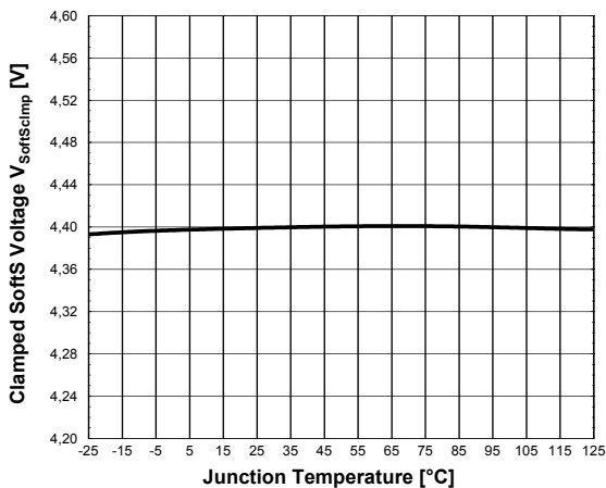
Figure 41 Clamped SoftS Voltage V_{SoftScImp}
