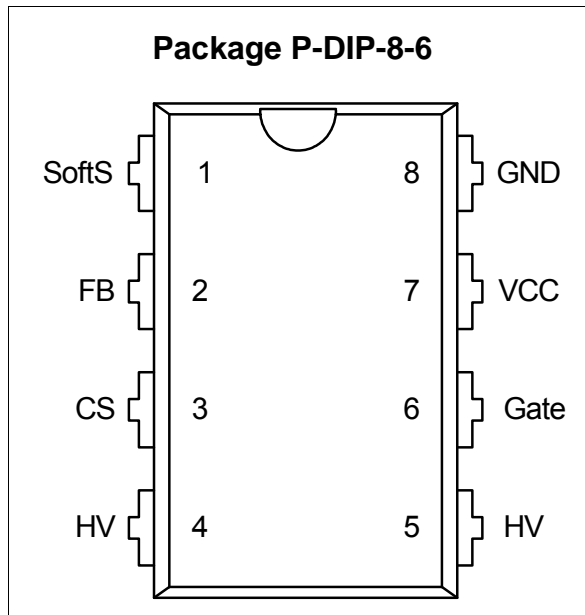
Figure 1 Pin Configuration P-DIP-8-6(top view)
