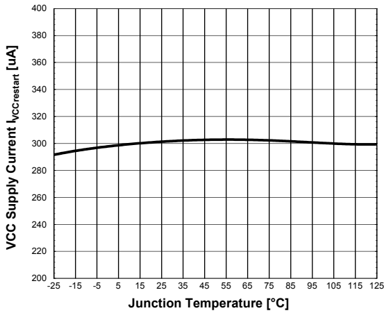
Figure 27 VCC Supply Current I_{VCCrestart}
