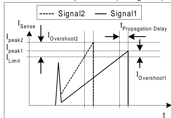
Figure 12 Current Limiting
