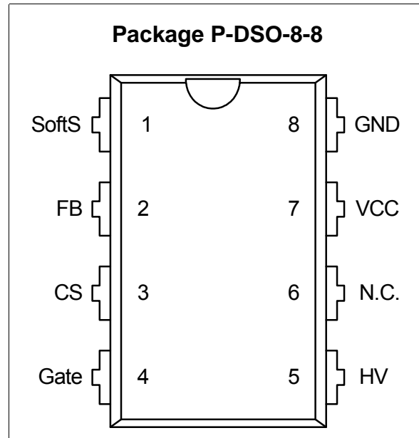
Figure 2 Pin Configuration P-DSO-8-8(top view)
