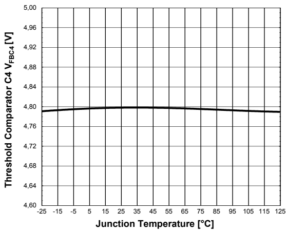
Figure 45 Threshold Comparator C4 V_{FBC4}
