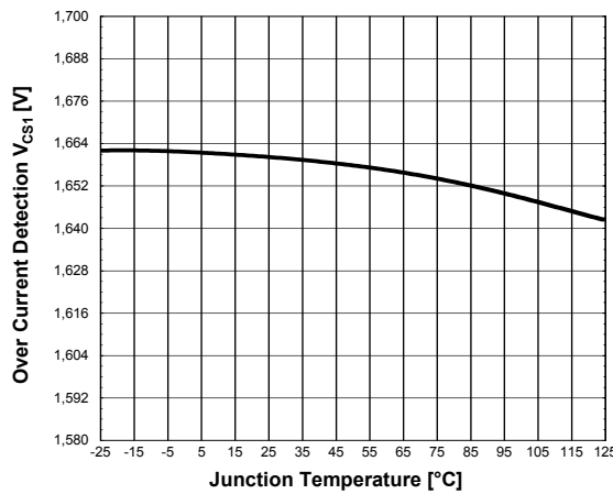
Figure 49 Over Current Detection V_{CS1}
