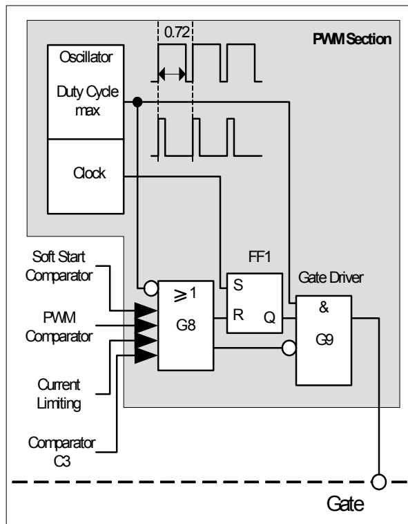
Figure 7 PWM Section
