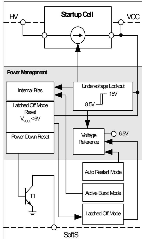
Figure 4 Power Management
