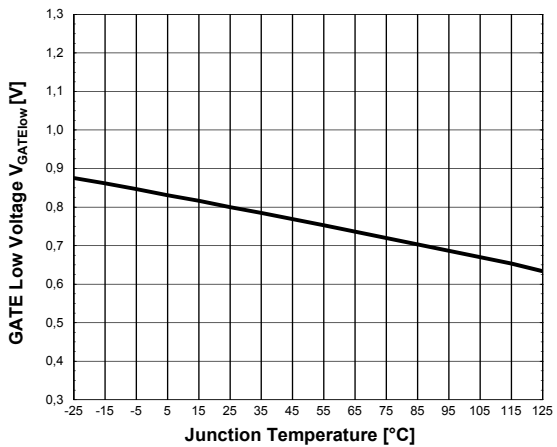
Figure 53 GATE Low Voltage V_{GATELow}
