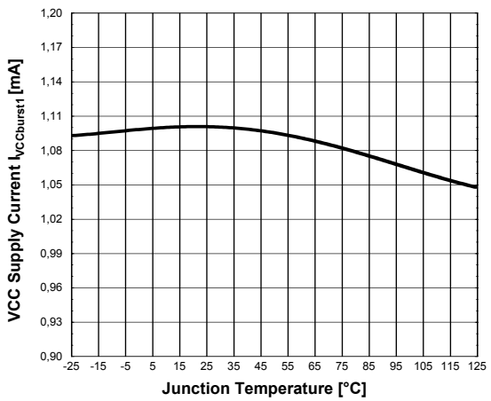
Figure 28 VCC Supply Current I_{VCCburst1}
