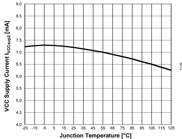
Figure 25 VCC Supply Current I_{VCCsup2}
