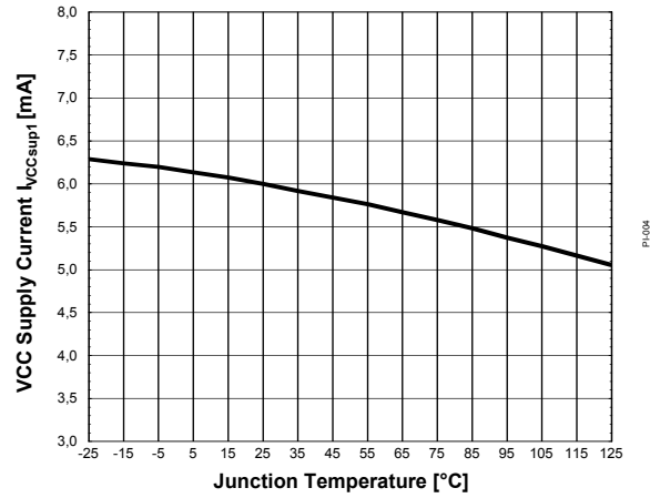
Figure 24 VCC Supply Current I_{VCCsup1}
