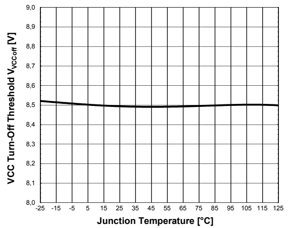
Figure 31 VCC Turn-Off Threshold V_{VCCoff}
