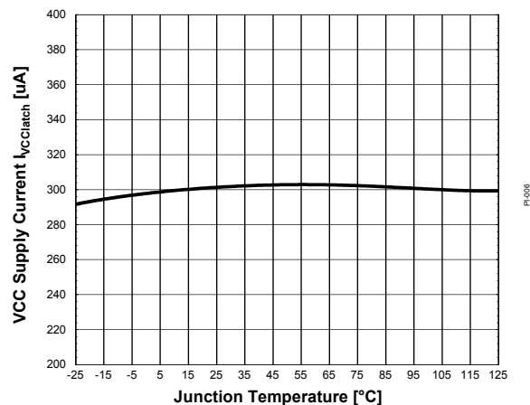
Figure 26 VCC Supply Current I_{VCClatch}
