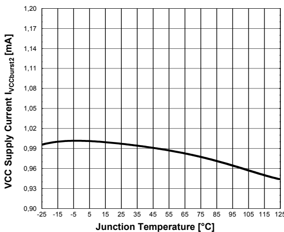
Figure 29 VCC Supply Current I_{VCCburst2}
