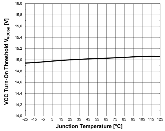
Figure 30 VCC Turn-On Threshold V_{VCCon}
