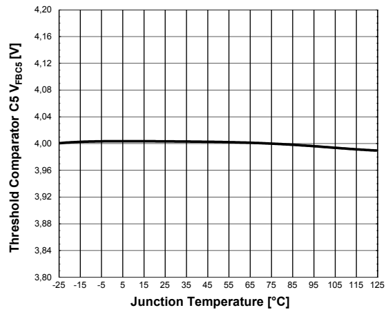
Figure 44 Threshold Comparator C5 V_{FBC5}
