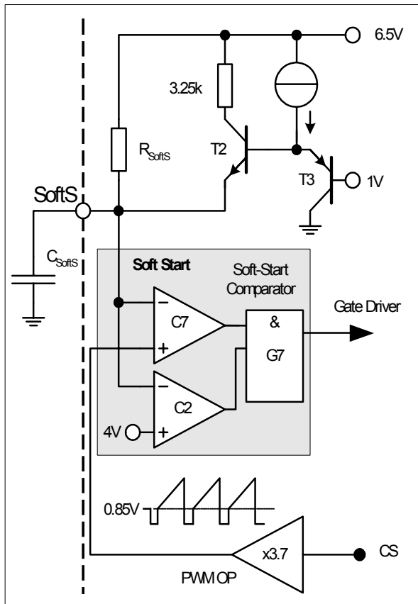
Figure 5 Soft Start
