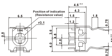
TSR-3318F FRONT VIEW
