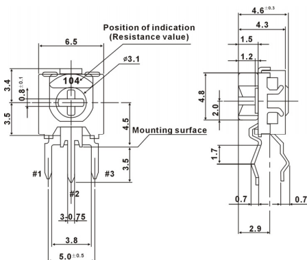
TSR-3318K FRONT VIEW
