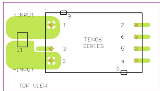
Recommended EN55022 Class B Filter Circuit Layout
