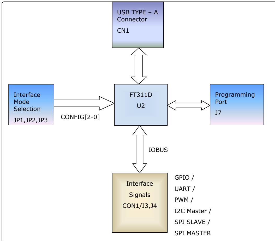
Figure 2.1 : FT311D Development Module Block Diagram
