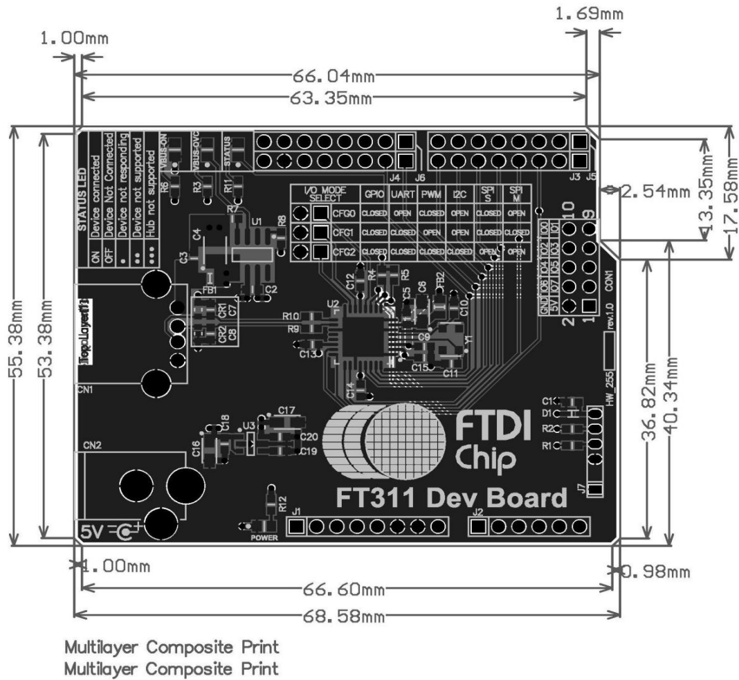
Figure 3.1 : FT311D Development Module Layout
