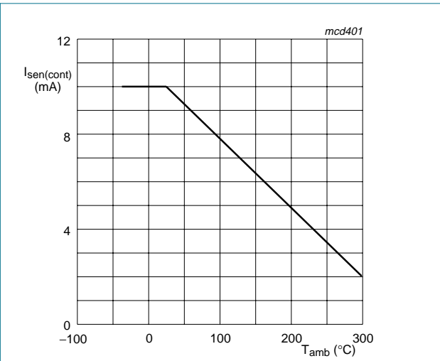
Fig 2. Maximum operating current for safe operation
