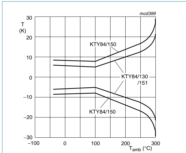
Fig 1. Maximum expected temperature error ( \Delta T )
