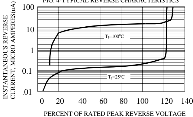
FIG. 4-TYPICAL REVERSE CHARACTERISTICS
