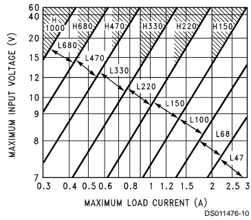
FIGURE 4. LM2576(HV)-5.0
