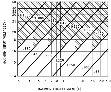
FIGURE 5. LM2576(HV)-12
