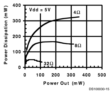
Power Dissipation vs Output Power
