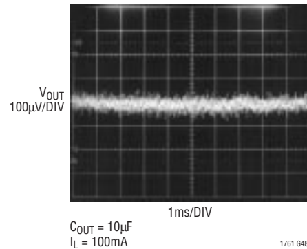
LT1761-5 10Hz to 100kHz Output Noise C_{BYP} = 0.01\mu F
