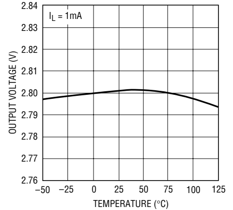
LT1761-2.8 Output Voltage
