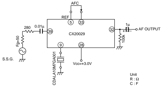
Test Circuit
