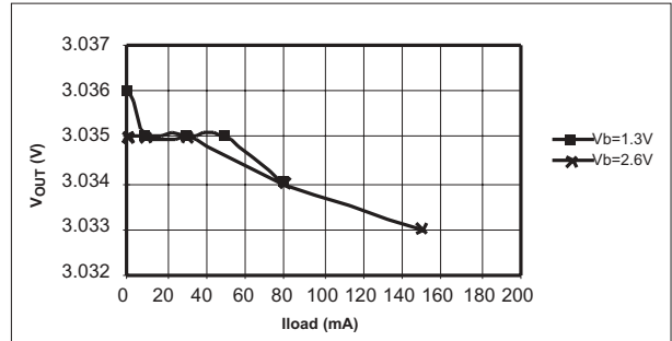
Figure 18. SP6644/6201 LDO Line/Load Rejection vs. Output Current ( V_{out}=3.3\text{V} ), R_{lim}=2.5\text{k} , L_i=22\mu\text{H} Sumida CD-43, Refer to Figure 30
