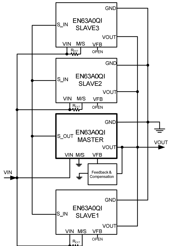
Figure 5: Master/Slave Parallel Operation Diagram
