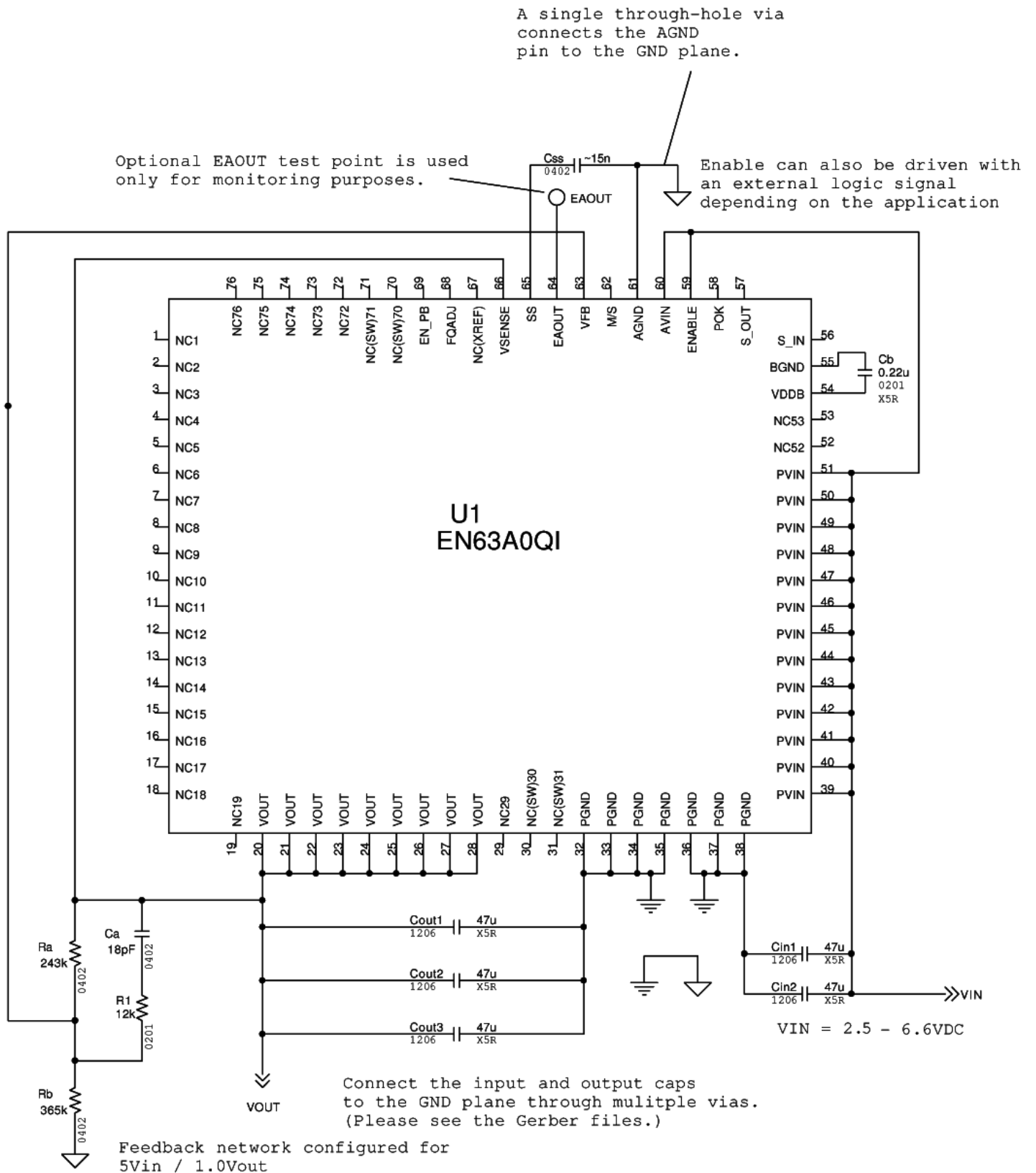
Figure 9: Engineering Schematic with Engineering Notes
