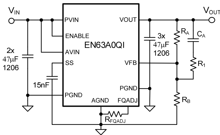
Figure 1. Simplified Applications Circuit
