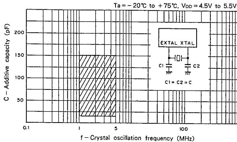
Fig. 10 Crystal oscillation circuit additive capacity calculation chart
