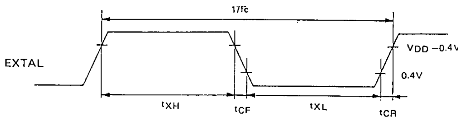
Fig. 1 Clock timing
