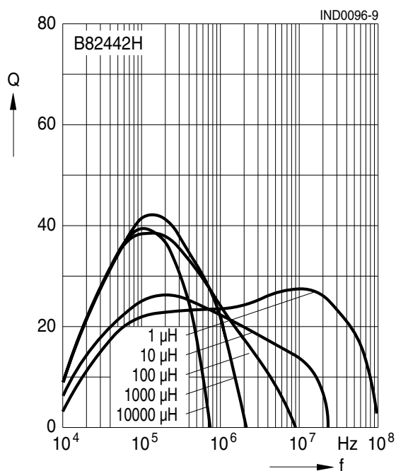
Q factor versus frequency f measured with impedance analyzer Agilent 4191A, typical values at 20 °C
