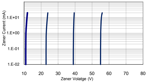
FIG 3 Zener Breakdown Characteristics
