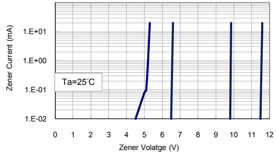
FIG 2 Zener Breakdown Characteristics
