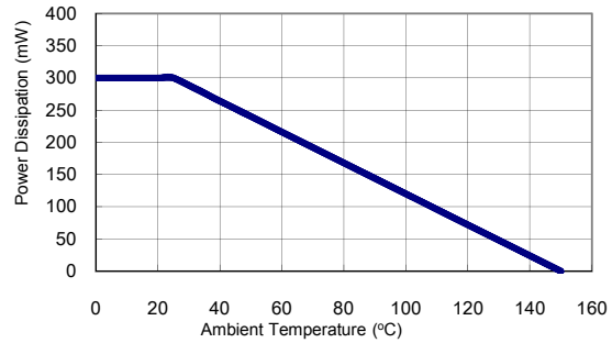
FIG 4 Admissible Power Dissipation Curve
