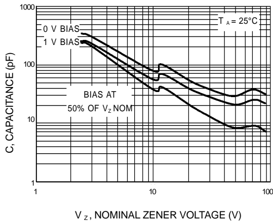
Figure 5. Typical Capacitance
