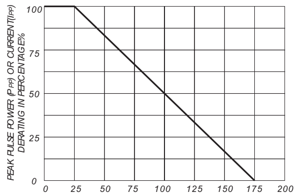
FIGURE 2 DERATING CURVE
