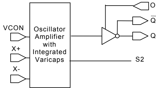
PLL520-8X Block Diagram
