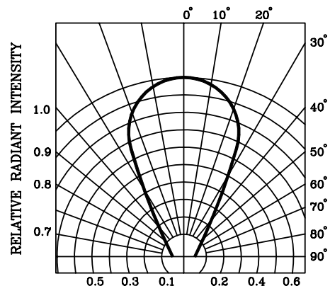
Fig.6 RADIATION DIAGRAM RADIATION DIAGRAM
