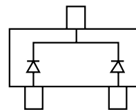
BAS70H-05 Marking: K75
