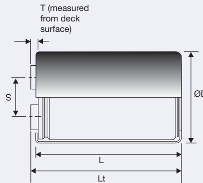
ALS36 Clamp Mounting
