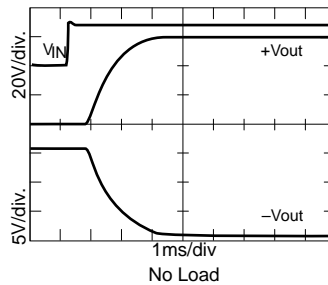
MFL2815D Turn On Response
