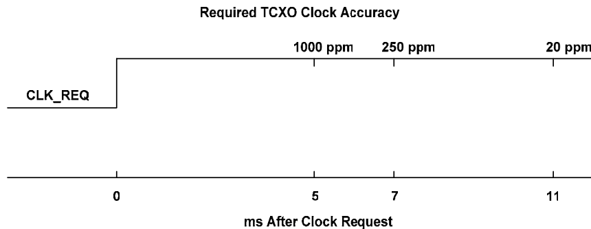
Figure 11.3: TCXO Clock Accuracy
