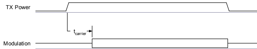
Figure 11.2: Internal Power Ramping
