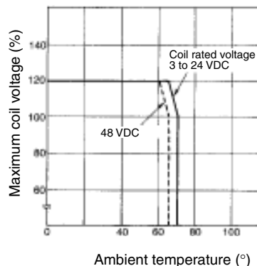
Ambient Temperature vs. Maximum Coil Voltage G5V-2
