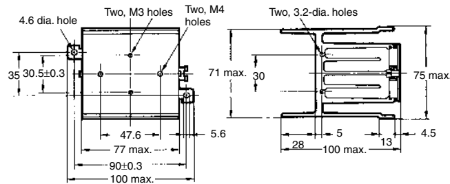
Mounting Holes
