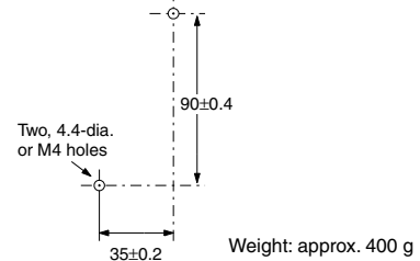
Mounting Holes
