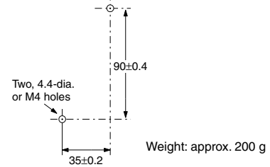
Mounting Holes
