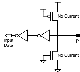
CMOS Pin (Input Mode) P xxoe = 0
