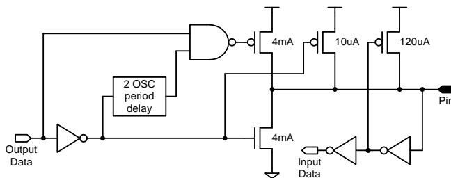
8051 Standard Pin
