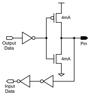
CMOS Pin (Output Mode) P xxoe = 1
