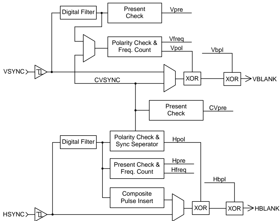
H/V SYNC Processor Block Diagram
