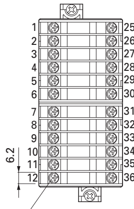
Terminal screw M3
