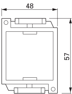
Mounting frame
