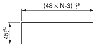
Side stick mounting (n units) (water-proof property is lost in this case)
