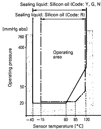
Fig. 1 Relation between sensor temperature and operating pressure
