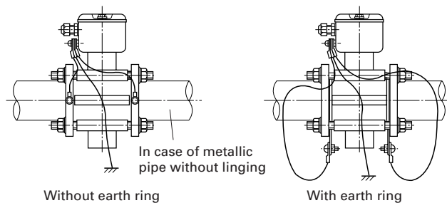
Grounding connection
