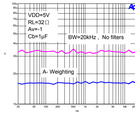
Output Noise
