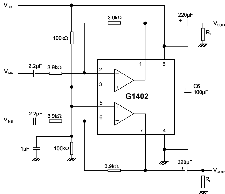
Fig.1 Measurement circuit for inverting application
