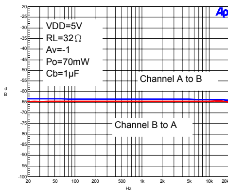
Channel Separation
